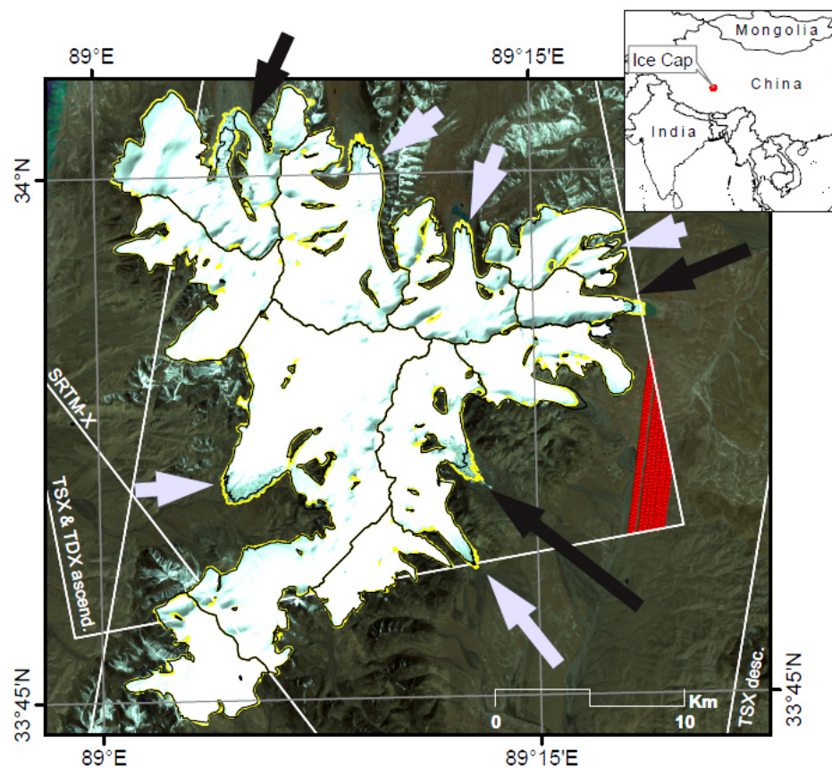
Fig. 1. Porogangri Icecap outlet glacier retreat 2000-2012 noted with black arrows for those with retreating more than 500 m and light purple arrows for those retreating less than 500 m.
