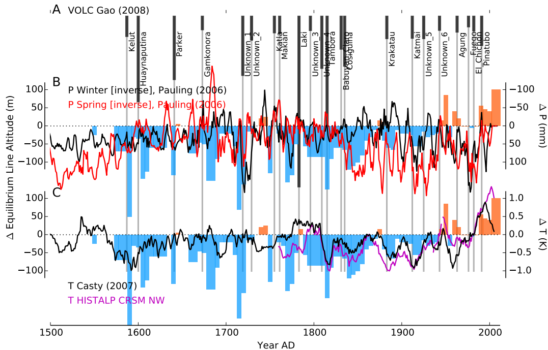
Fig. 1. Modeled ELAs are shown with red and blue colored areas. Instrumental records are shown for comparison in panels (B) and (C). Precipitation from Pauling et al. (2006) is smoothed
