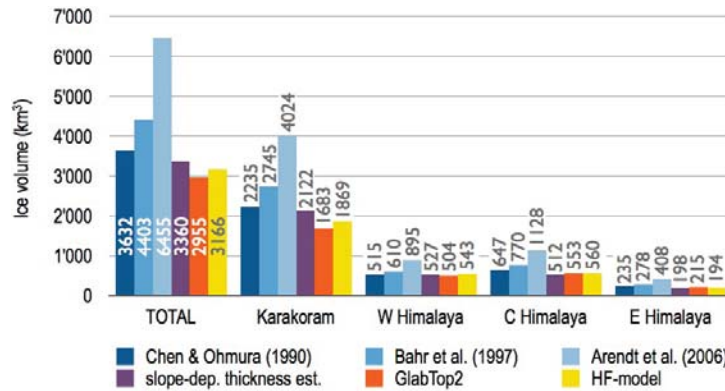
Fig. 5. Resulting volumes ( km^3 ) for the entire HK region (left) and the four sub-regions.
