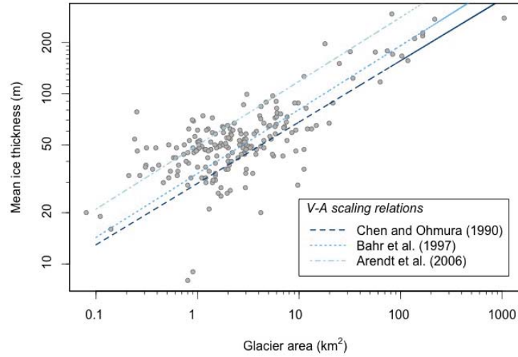
Fig. 8. Mean thickness vs. glacier area for “measured” glaciers, including the scaling relations used in this study. Note the variability of mean thickness of up to an order of magnitude for a given glacier size. (Data collected by Graham Cogley and Regine Hock, published in Cogley, 2012, downloaded from Grinsted, 2013).
