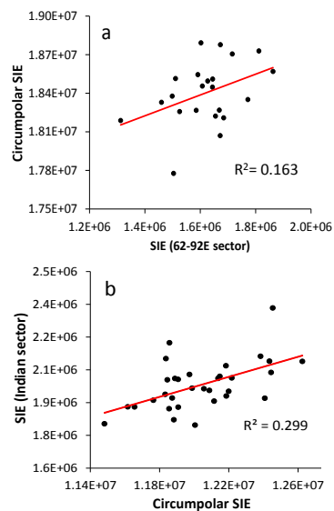
Figure 5. The linear correlation between SIE at (a) the sector highest-correlated with LGB69 MS- (62°E–92°E), and (b) the whole Indian Ocean sector (30°E–105°E) with the total circum-Antarctic SIE for August to October, 1979–2000 (unit: km 2 ).
