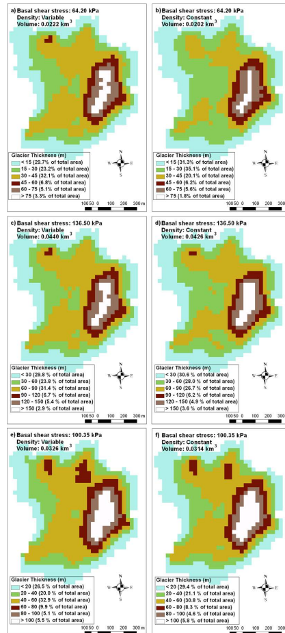
Fig. 1. Quayna West glacier thickness considering different values of basal shear stress, constant glacier density and variable glacier density.
