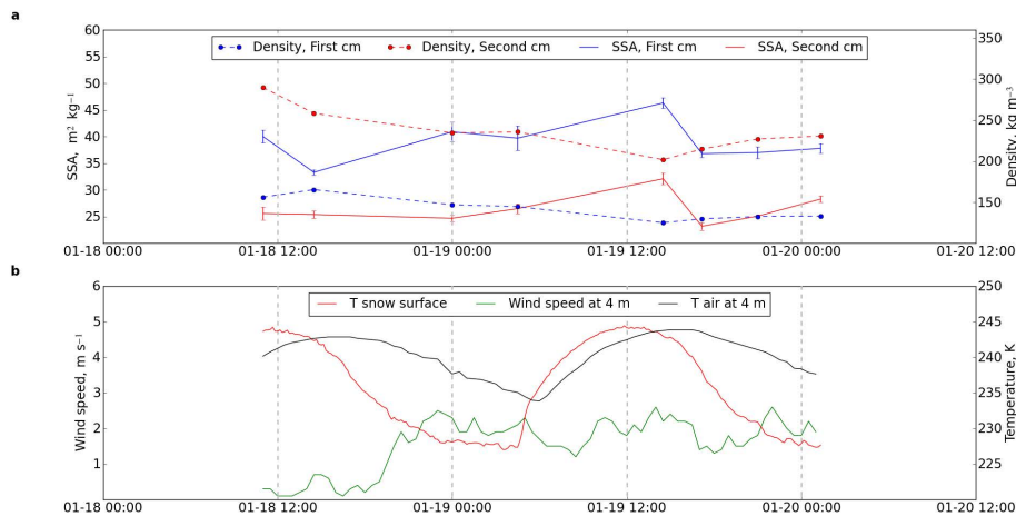
Fig. 2. Time series of physical variables on 18 and 19 January 2009. Time is local time, GMT + 08:00. (a) Snow SSA and density values. (b) Meteorological variables.
