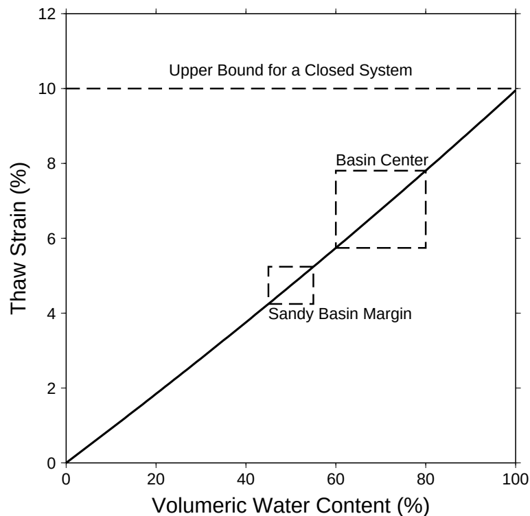
Fig. 5. Theoretical relation between the thaw strain and the volumetric water content when freezing and thawing of the soil occurs in a closed system. Thaw strain has an upper bound of 10%. The two boxes outline the ranges of thaw strains and volumetric water contents for the sandy margins and the center of the basin, respectively.
