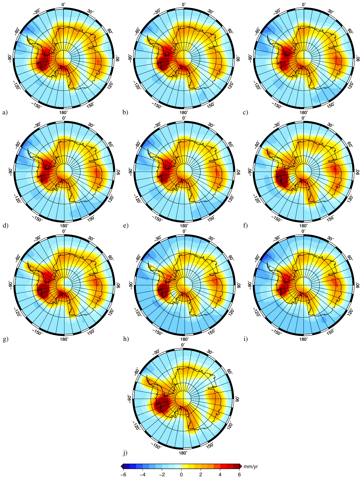
Fig. S2. Estimated GIA vertical rates computed from the following GRACE solutions: a) CSR RL04, b) CSR RL04 DDK3, c) CSR RL05, d) CSR RL05 DDK5, e) CSR RL05 Regularized, f) GFZ RL04, g) GFZ RL04 DDK3, h) GFZ RL05, i) GFZ RL05 DDK5, j) DMT-1b
