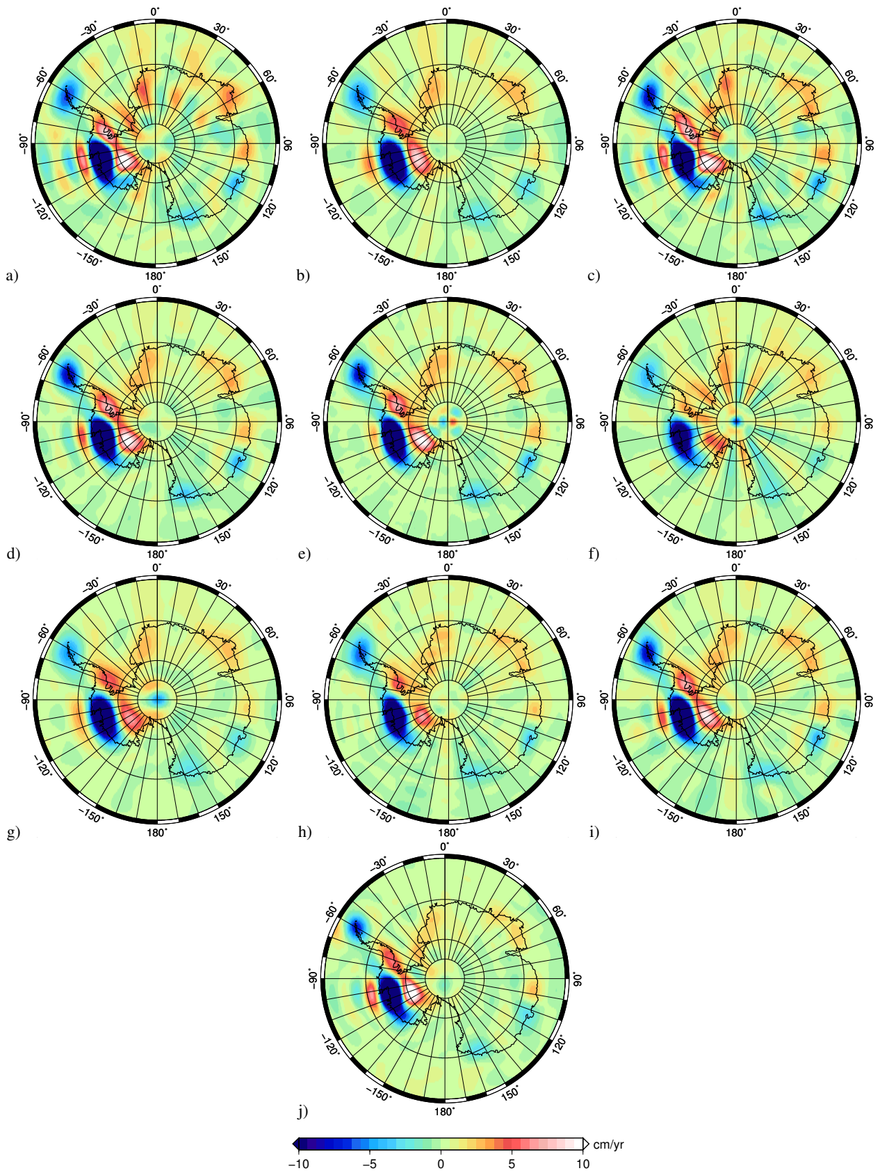
Fig. S1. Mass change trends of the following GRACE solutions, in units of EWH: a) CSR RL04, b) CSR RL04 DDK3, c) CSR RL05, d) CSR RL05 DDK5, e) CSR RL05 Regularized, f) GFZ RL04, g) GFZ RL04 DDK3, h) GFZ RL05, i) GFZ RL05 DDK5, j) DMT-1b
