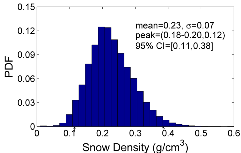
Fig. 10. Probability distribution function (PDF) of snow density for all data. The bar is PDF of snow density; the arrows bracket 2.5% and 97.5% spectrum distribution of snow density. Mean and \sigma represent the calculated mean and standard deviation of all snow density, respectively. Peak stands for the peak PDF of snow density (right) and the corresponding snow density (left). 95% CI is 95% credibility intervals of snow density that lie between 0.11 and 0.38 g cm -3 .
