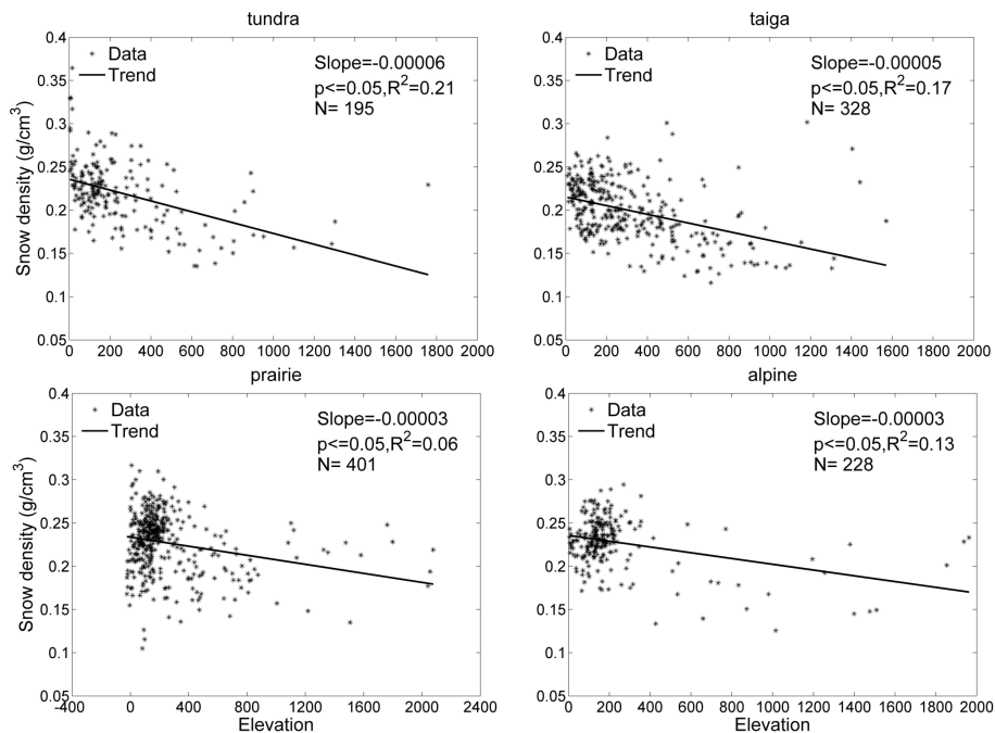
Fig. 14. Same as Fig. 13, but for tundra, taiga, prairie, and alpine snow.
