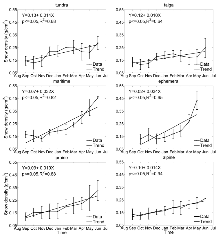
Fig. 6. Monthly mean snow density for tundra, taiga, maritime, ephemeral, prairie, and alpine snow. The attributions were the same as Fig. 5.
