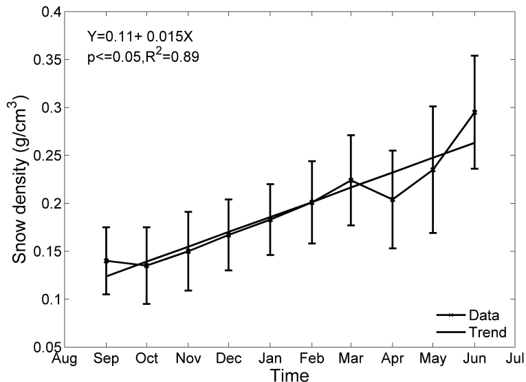
Fig. 5. Monthly mean snow density at 1259 stations across the former USSR from 1966 to 2008. The asterisk is the computed monthly mean snow density; the error bar represents one standard deviation from the mean. The thick line is a linear regression trend. Y-axis stands for snow density in \text{gcm}^{-3} , and x-axis for time in months (from September to June), p is the confidence interval for the coefficient estimates, and R^2 is the sum of residual squares. September was the first month in a snow cover year, therefore, X ranged from 1 (September) to 10 (June) in the simulation of monthly snow density.
