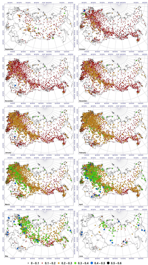
Fig. 4. Spatial distribution of monthly mean snow density for each station during 1966 to 2008 across the former USSR. Dot represents the value of the monthly mean snow density ( \text{g cm}^{-3} ) of each station.
