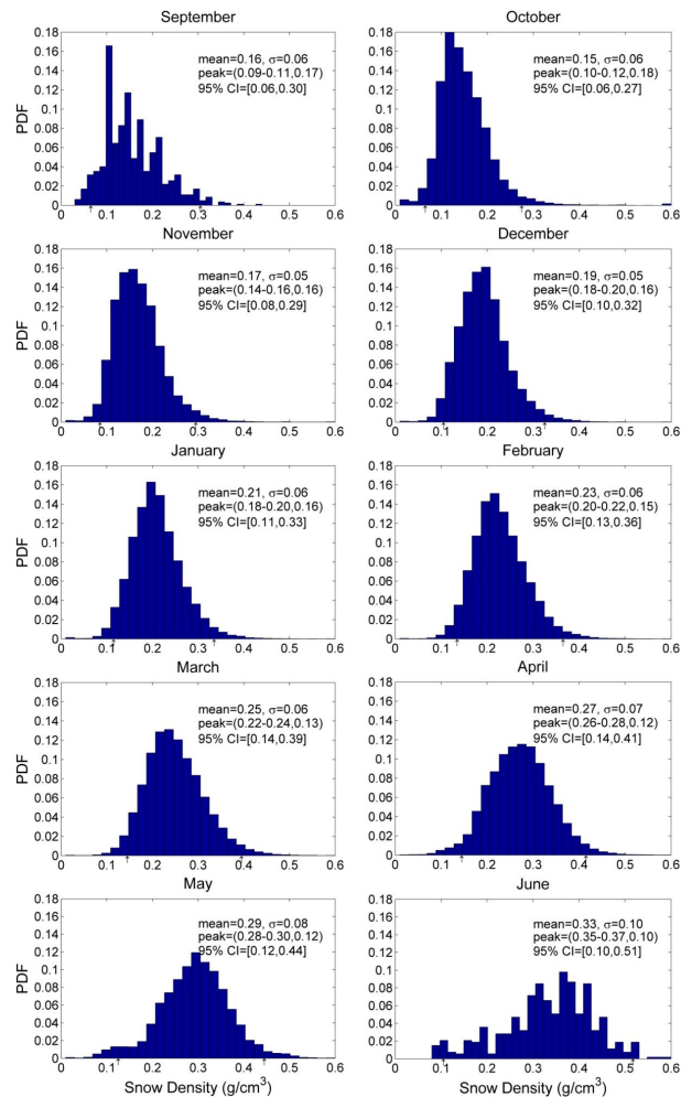
Fig. 12. PDF of monthly snow density. The attributions were the same as Fig. 10.
