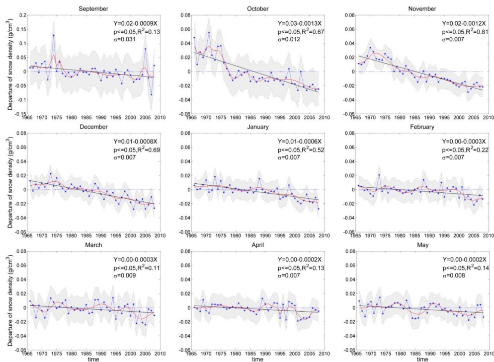
Fig. 8. The annual variation of monthly snow density across the former USSR from 1966 through 2008, with respect to the 1971–2000 mean. The attributions were the same as Fig. 7.
