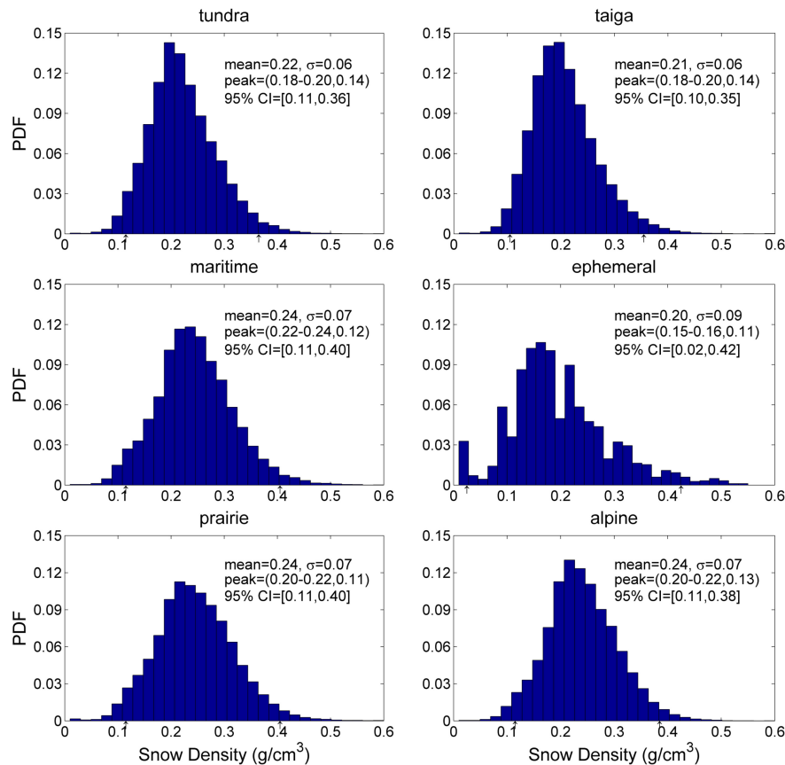
Fig. 11. PDF of snow density for tundra, taiga, maritime, ephemeral, prairie, and alpine snow. The attributions were the same as Fig. 10.
