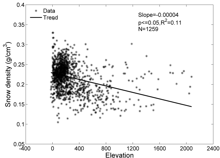
Fig. 13. Snow density changes with elevation for all stations across the former USSR during 1966–2008. Asterisk shows the mean snow density of each site; the thick line is a linear regression with the parameters shown on the upper-right corner, where slope was -0.004 in \text{g cm}^{-3} - 100 \text{ m} , p is the 95% confidence intervals for the coefficient estimates, R^2 is the sum of residual squares, and N is the number of stations.
