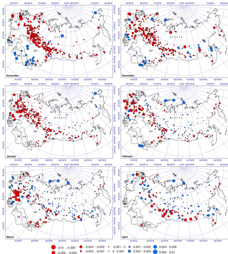
Fig. 9. Spatial distributions of linear trend coefficients ( \text{gcm}^{-3} \text{yr}^{-1} ) of monthly mean snow density (from November to April) for each station during 1966–2008. The rates of changes in monthly mean snow depth were statistically significant at > 95 % significant level. Red circle represents decreasing trend, and blue one is increasing trend.
