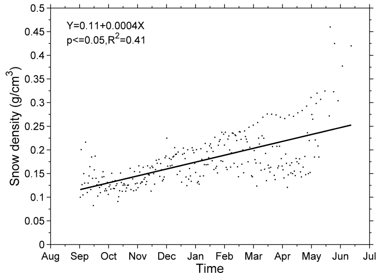
Fig. 3. Daily mean snow density at all stations across the former USSR from September to June. The dot is the computed daily mean snow density of all stations. The thick line represents a linear regression trend. Y-axis stands for snow density in \text{g cm}^{-3} , and x-axis for date; p is the confidence interval for the coefficient estimates, and R^2 is the sum of residual squares. We defined 1 September as the first day in a snow cover year, therefore, X ranged from 1 (1 September) to 304 (30 June) in the simulation of daily snow density.
