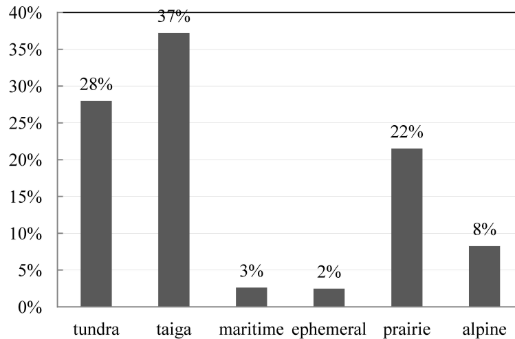
Fig. 2. The percentage of snow cover area for six snow classes across the former USSR.
