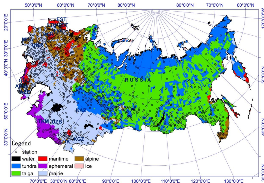
Fig. 1. Geographical locations and distribution of snow course stations and snow classes.
