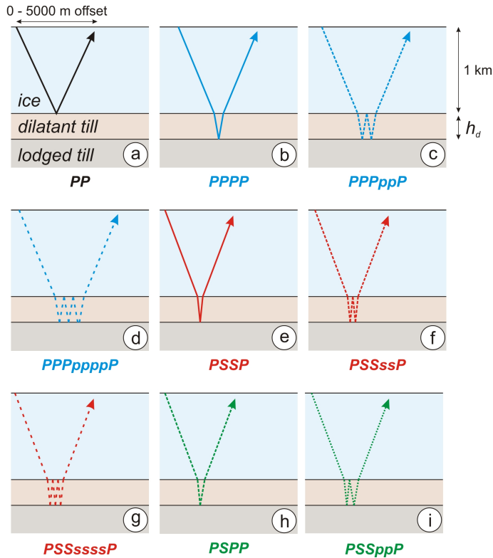
Fig. 2. Nomenclature and schematic representation of raypaths considered in modelling. Line colours and styles are equivalent to those in successive figures. Raypath (a) is the basal ice reflection (black), (b–d) comprise P-wave propagation along the whole travel-path (blue), (e–g) have S-wave mode conversions within the dilatant till (red), and (h) and (i) convert between S and P-wave modes within the dilatant till (green).
