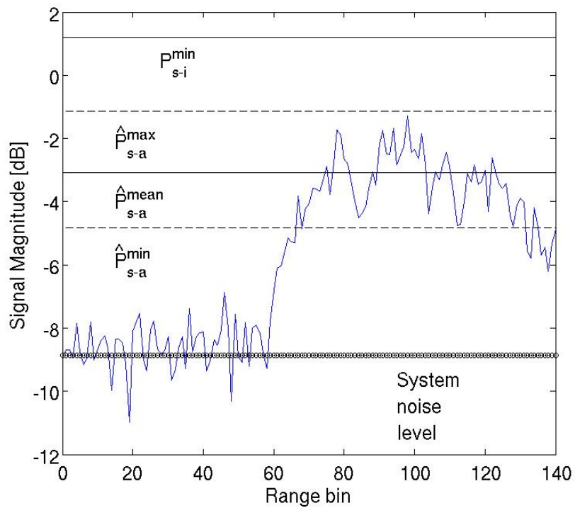
Fig. 3. Example radar waveform over a ridge. The point of maximum power in the radar waveform is within the expected range for the snow-air interface and does not reach the minimum required threshold.
