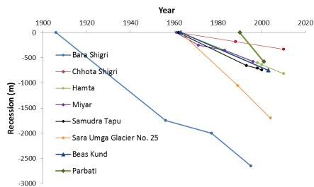
Figure : Snouts fluctuations in Himachal Pradesh. Most of the data have been performed at decadal resolution (or more) and are not helpful to detect a balanced or slightly positive mass budget during the nineties.
