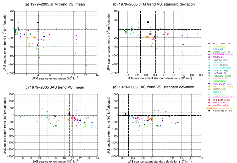
Fig. 3. Sea ice extent trend for the period 1979–2005 over the whole Southern Ocean vs. mean ( a, c ) and standard deviation ( b, d ). The first row corresponds to summer (JFM), the second to winter (JAS). The different colors correspond to the historical simulations from 24 different models. For each color, the small dots refer to model individual members and the symbol specified in the legend is for the model ensemble mean. The number of members in each model is indicated in brackets in the legend. Orange refers to multi-model means; diamond sign is for the average over all the models, circle sign is for the mean of models with interactive chemistry (in bold in Table 2) and triangle sign is for the mean of models with 35 atmospheric levels or more on the vertical. Black square is for the observations (Cavalieri and Parkinson, 2008), surrounded by 2 standard deviations (black dashed lines).
