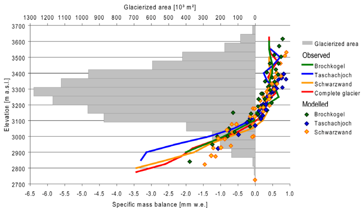
Observed (line) and modeled (squares) specific mass balance in four parts of the Vernagt glacier for the elevation levels in the mass balance season 1999 (Marowsky (2010), p. 78, modified).
