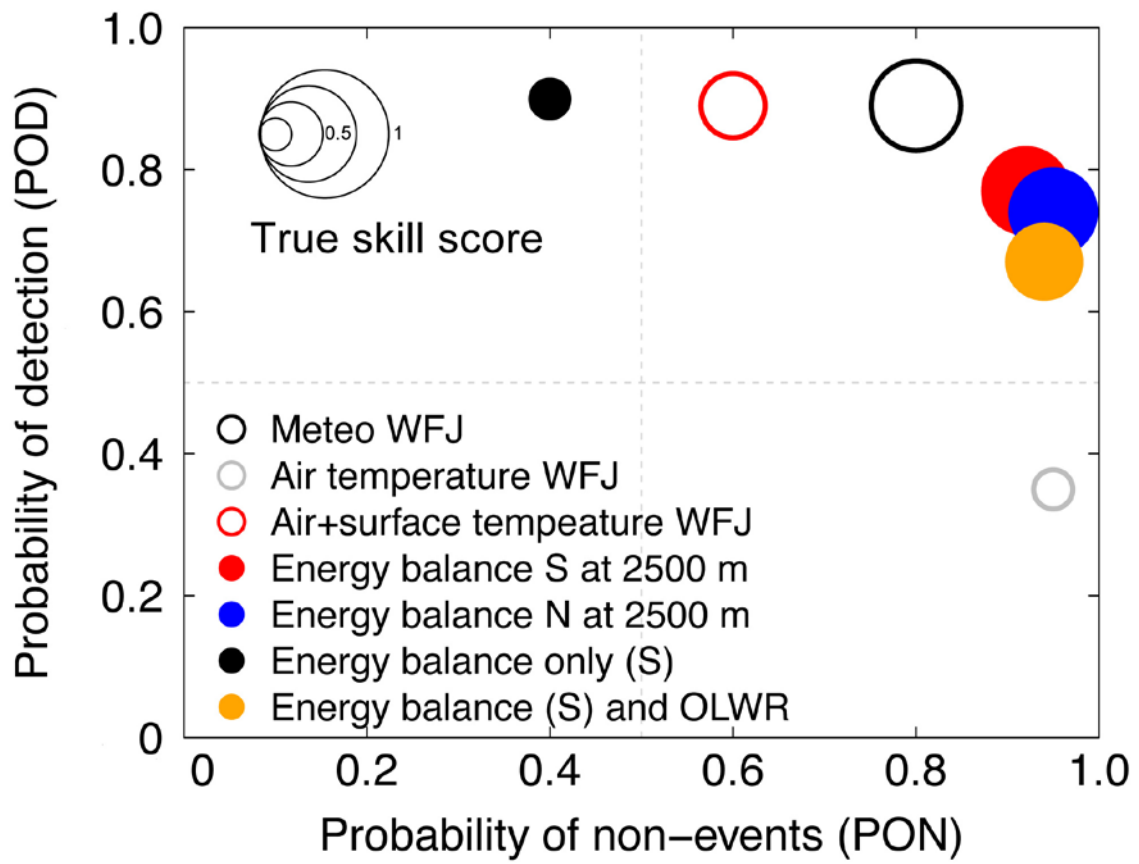
Figure 2: Predictive skills of various classification tree models. Size of the circles represent the true skill score.
