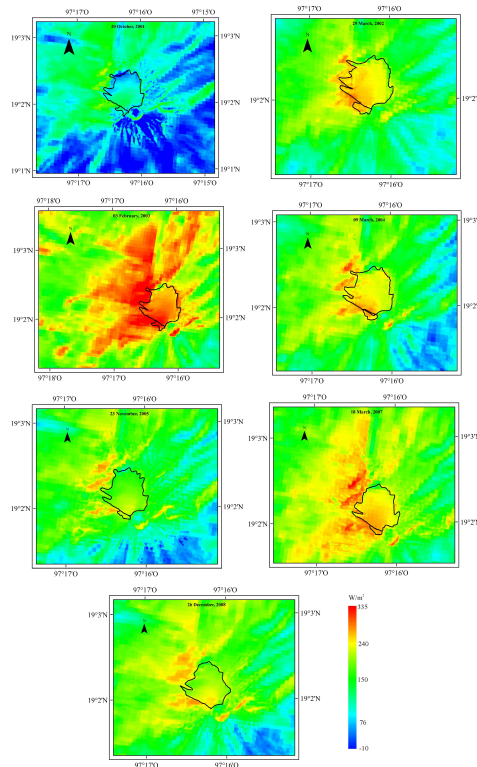
Fig. 6. Net radiation distribution over Glaciar Norte's surface derived from ASTER imagery. The highest values are observed in February 2003 and March 2007. In almost images is possible to observe the
