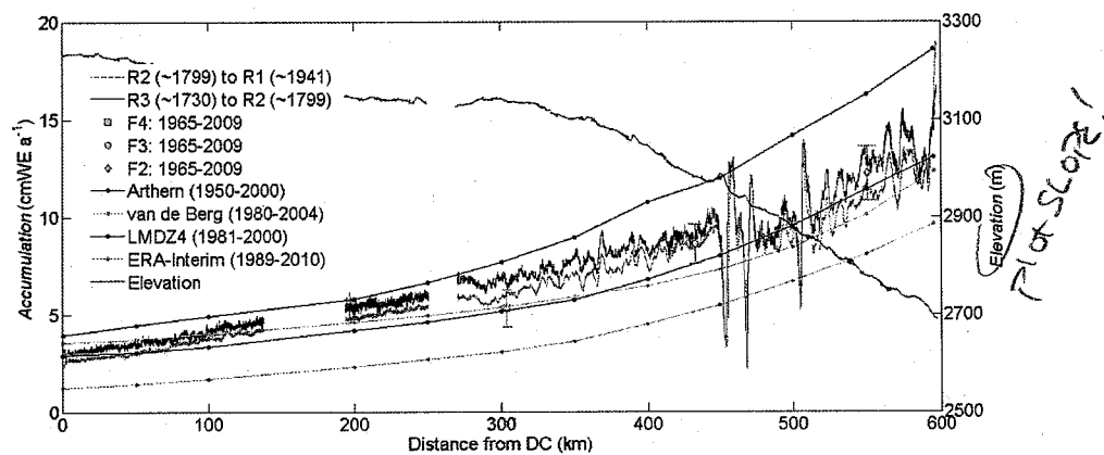
Fig. 9. Comparison between our accumulation results (radar and core measurements) and modeling results along the transect.
