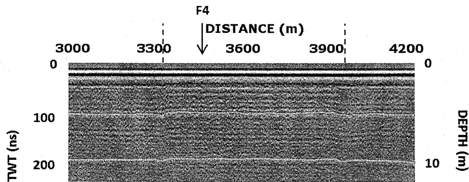
Fig. 4. Transition between “real” and “natural” snow surface visible on radagram 9 in the vicinity of core F4. The first dotted line corresponds to the point where the radar vehicle left the traverse route and the second one to the point where it got back to the traverse route.
