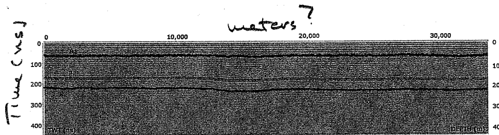
Fig. 2. Picked reflectors labeled R1 to R3 shown on radargram 5. Distance is in meters
