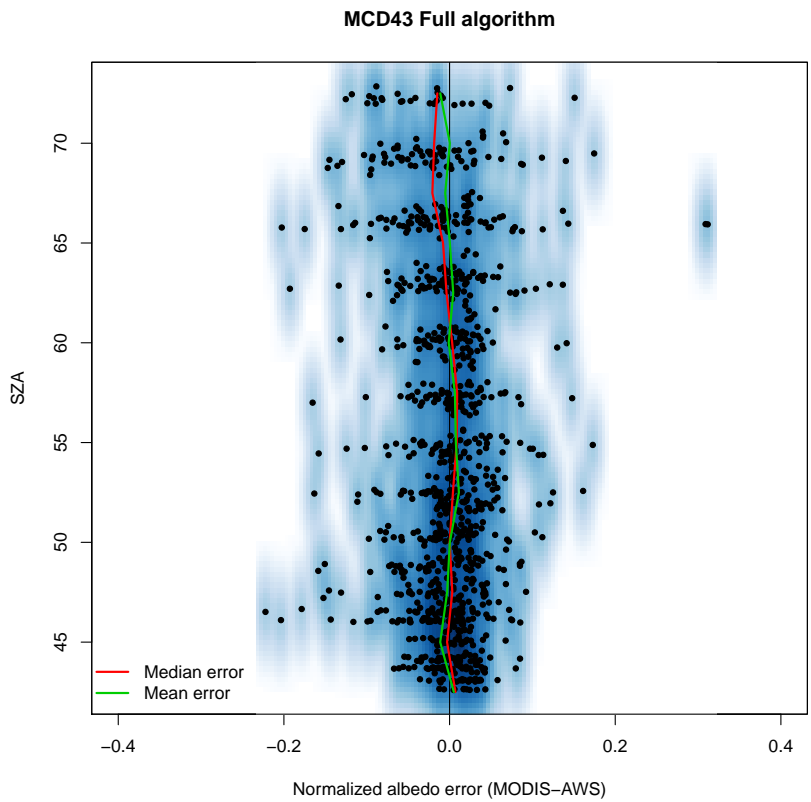
Figure A 2. Same as Figure A1, but for the 16 day integrated full algorithm MCD43 product.
