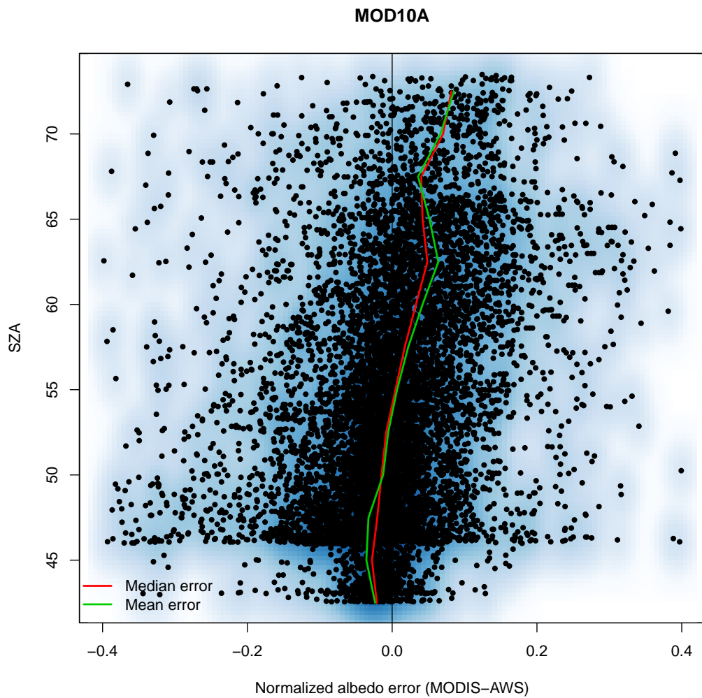
Figure A 1. Difference between the MOD10 daily albedo product and AWS measurements as function of solar zenith angle (SZA).
