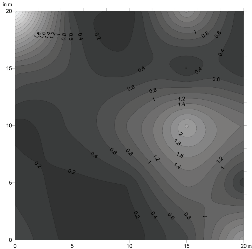
Fig. 8. Contour plot of the spatial distribution of ikaite in the first 10 cm of land fast sea ice off Terre Adélie (DDU) in November 2007 on a 20 m × 20 m grid with sample points every 5 m. Values are in mg ikaite l -1 melted sea ice.
