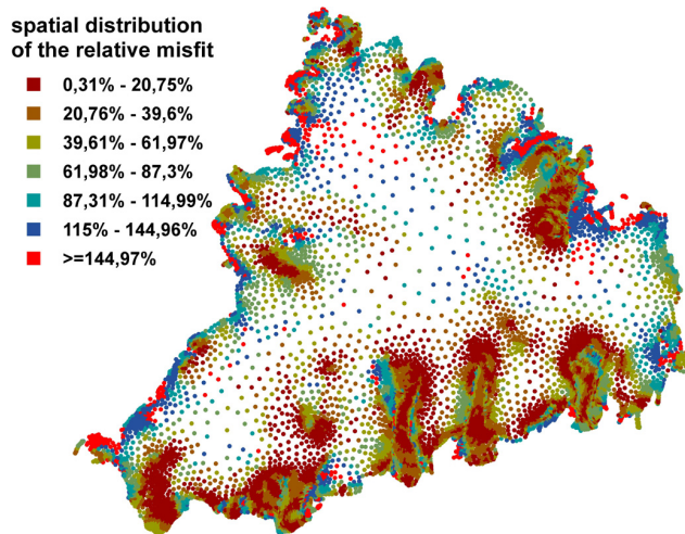
Fig. 9. Spatial distribution of the relative misfit between Neumann and Dirichlet velocities over the whole glacier surface. Comparison with Fig. 8 indicates that relative errors are similar in the fast-flow and slow-flow regime areas. The points with relative errors higher than 145 % are highlighted in red to demonstrate that these are single points, mostly close to the margins.
