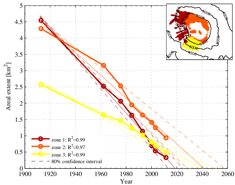
Fig. 5. The areal change of glaciers and ice bodies based on the three member classification. Linear regressions (solid lines) for each of the three zones are shown, as well as the 80 % confidence intervals for each of these relationships.
