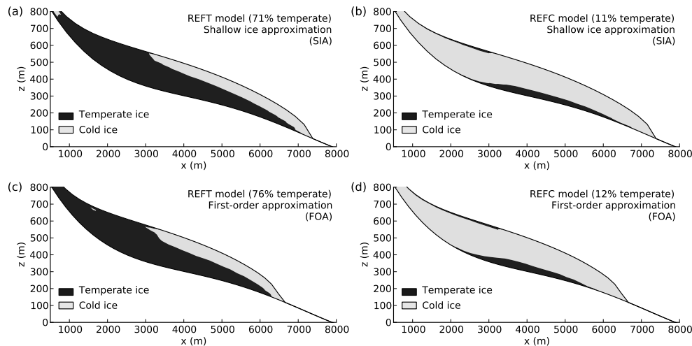
Fig. 2. Distribution of cold and temperate ice in reference models REFT and REFC with the shallow ice approximation (a, b) and the first-order approximation (c, d) for ice dynamics. Prescribed mean air temperature T_{ma} is lowered by 1.5 K in REFT to obtain REFC. For REFC, the glacier ice surface is held fixed at the REFT geometry.
