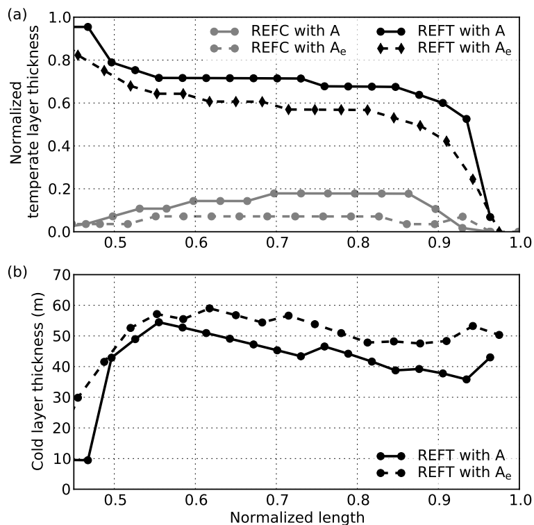
Fig. 4. Effect of flow-law coefficient parametrization on glacier thermal structure. Glacier geometry evolves in these simulations. The basal temperate layer thickness (a) is normalized to ice thickness. The cold layer thickness in (b) is equivalent to the cold-temperate transition depth.
