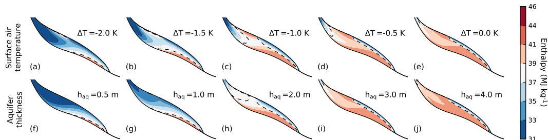
Fig. 7. Examples of polythermal structure types in the model results. In the upper row ( a–e ), surface air temperature ( \Delta T ) is varied. In the lower row ( f–j ), near-surface aquifer thickness ( h_{\text{aq}} ) is varied. Each panel represents a steady-state. Dashed line indicates the cold-temperate transition.
