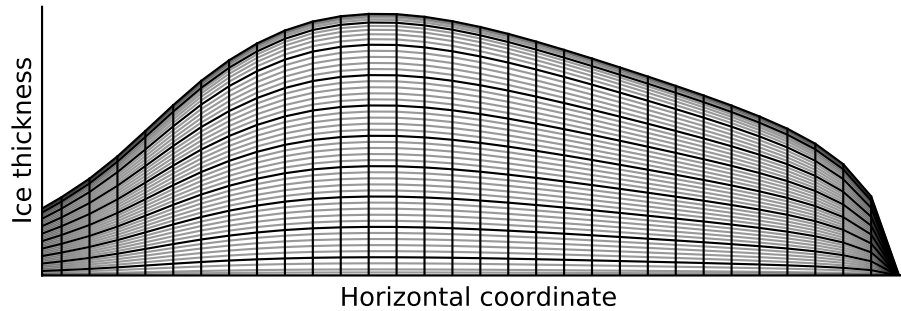
Fig. 1. The structured model domain for the finite-difference scheme, shown in terms of ice thickness for visibility. The uppermost cell height is 0.5 m. Cell height increases linearly in the upper 10 layers and then remains constant at a value that depends on ice thickness. The lowermost two cells are thinner to improve the modelled diffusion of heat into the basal layers.
