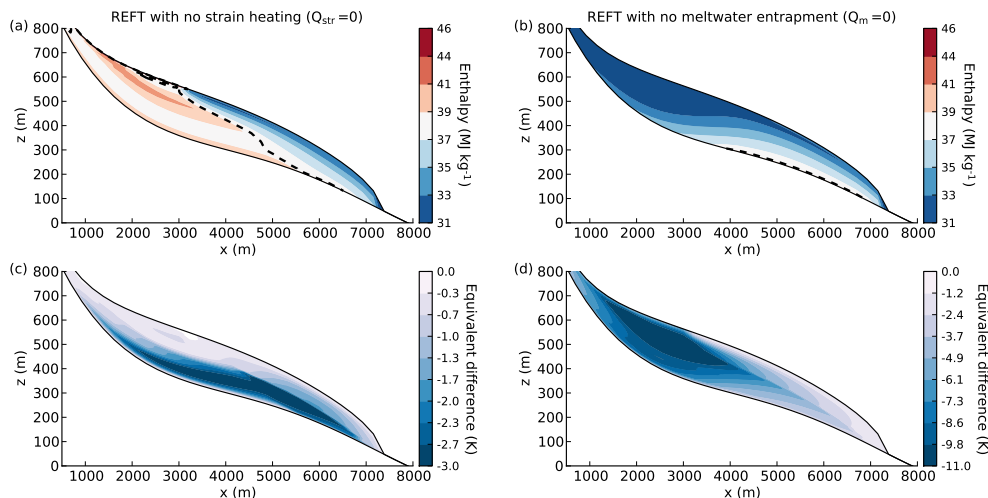
Fig. 3. Distributions of enthalpy and equivalent temperature difference ( \Delta K' ) for REFT with and without strain heating Q_{\text{str}} ( a, c ) and meltwater entrapment Q_m ( b, d ). Model runs use flow-law coefficient A as in Eq. (13). The dashed lines in ( a, b ) denote the cold-temperate transition. Darker areas in ( c, d ) indicate the largest differences in ice enthalpy relative to the REFT reference model. Shaded contours in ( c, d ) show the equivalent temperature difference for cold ice ( \Delta K' ) in units of Kelvin (Eq. 22).
