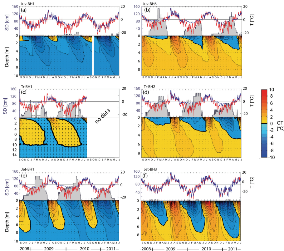
Fig. 3. Thermal regime of permafrost and non-permafrost borehole sites at Juvvasshøe ( a, b ), Tron ( c, d ) and Jetta ( e, f ) comprising GT, GST, T_{\text{AIR}} and snow depth (SD). The upper panel in each figure shows T_{\text{AIR}} (red line), GST (blue line) and SD (grey area). The lower panel in each figure represents a depth-time diagram of GT.
