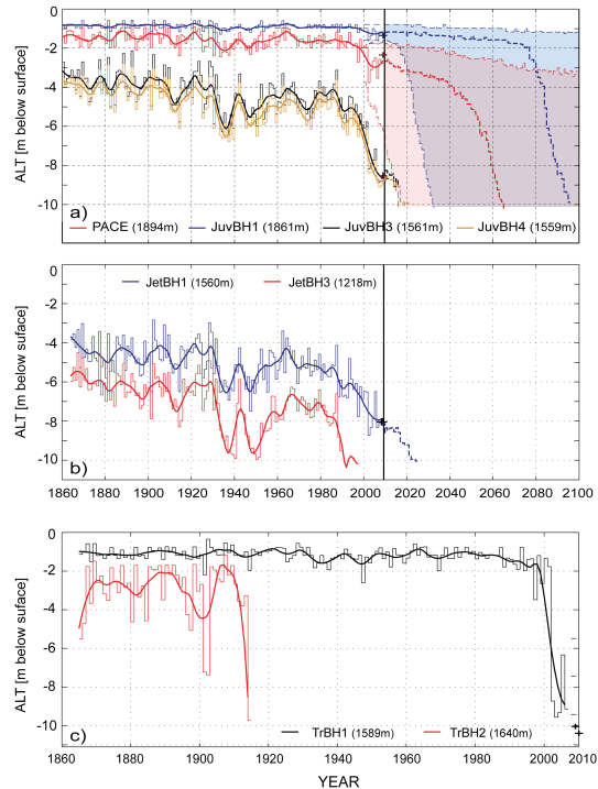
Fig. 9. Reconstructed and projected active layer thickness (ALT) from 1860 to 2100 at Juvvasshøe (a) , Jetta (b) and Tron (c) . Projected ALT was modelled using the ensemble-median T_{AIR} (bold dashed lines). For Juv-BH1 and PACE, also shown are ALT according to the 90 and 10 percentiles (shading) of the T_{AIR} ensemble. (a) . The bold lines represent a 7-yr Gaussian-filtered series, measured ALT are marked by crosses. The model indicates the permafrost degradation at Tron by the year 2010. Therefore, no projection was applied for Tr-BH1.
