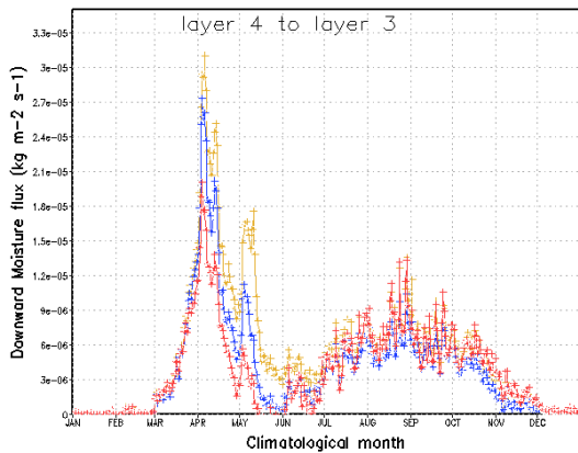
Fig. 8. Daily average downward moisture fluxes within the soil column over the Ob. A plot of climatological, area-average values over model runs for 1989–1999. Layer 4 is the top layer and layer 1 is the bottom.
