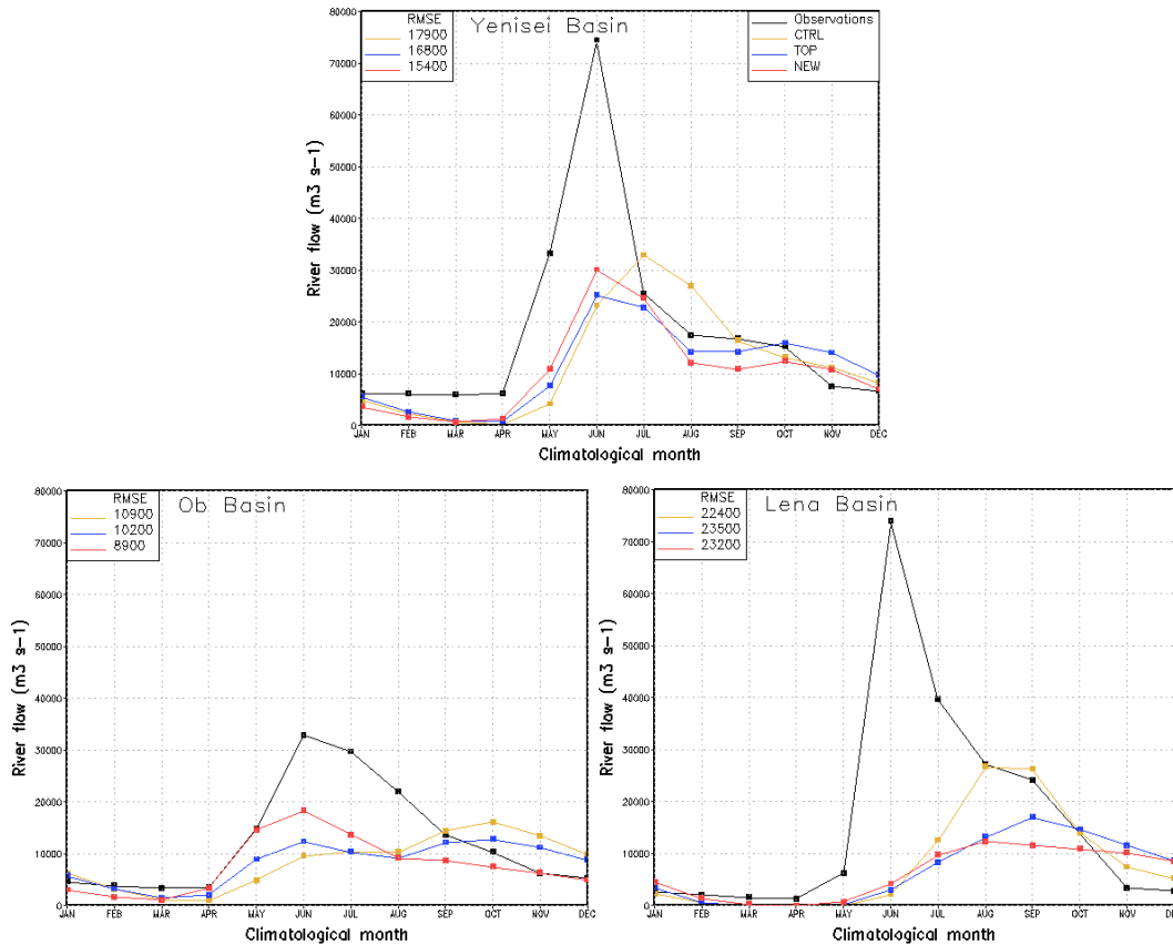
Fig. 5. Observed river flow of the Yenisei, Ob and Lena compared to model runs for each using CTRL, TOP and NEW. The points represent the average flow rate for a given month. Each observational point is a climatological average value of 60 consecutive years in the range 1930–1999, depending on the basin. The model points are a climatological average value for the decade 1989–1999. The RMSE values are the yearly-average values.
