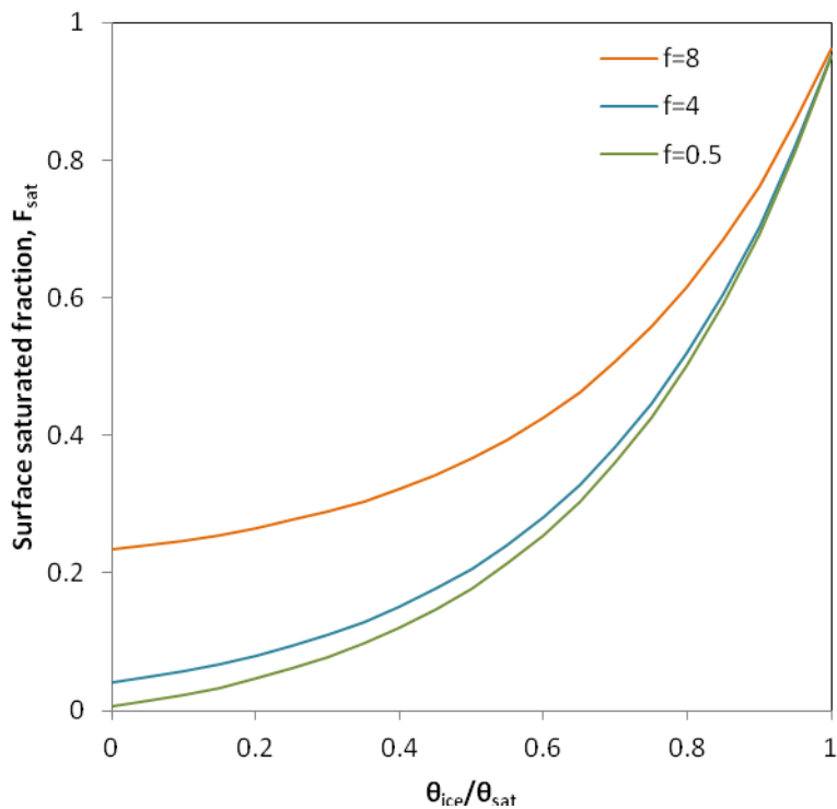
Fig. 2. Demonstrating the effect of f on the F_{sat} function. The maximum surface saturation value has been set to an approximate value of 0.3, mean water table depth has been set to 1 m and \alpha set to its chosen value of 3.0. The blue line uses the chosen model parameter while the orange and green lines use parameters that lie just outside the extremes of the selected parameter space.
