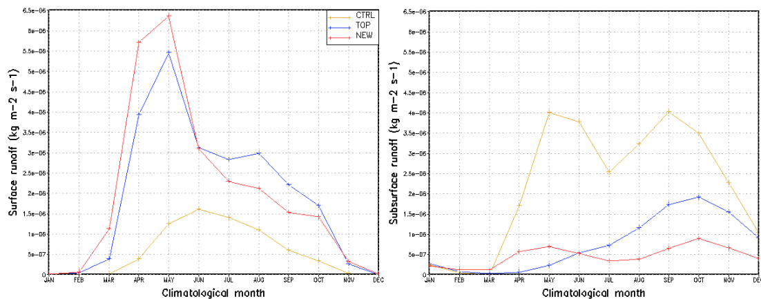
Fig. 7. Average monthly surface and subsurface runoff over the Ob. This is a plot of climatological, area-average values over model runs for 1989–1999.
