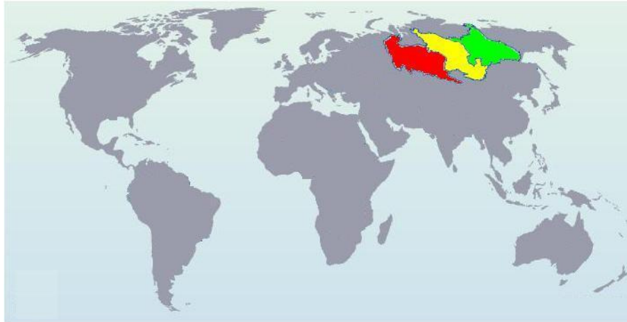
Fig. 4. Siberian river basins used in the investigation (UNEP/GRID-Arendal, 2002). In red is the Ob, in yellow is the Yenisei and in green is the Lena. This author has edited the colours and removed other basins that were in the image.
