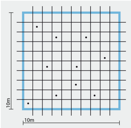
Fig. 4. Ten iButtons were randomly distributed in each 10 m×10 m footprint. One vertex of the square was marked with a stick. Two ropes representing two orthogonal edges were attached to the stick. The blue ropes served as rulers. The local grid and the sampled numbers were manually recorded.
