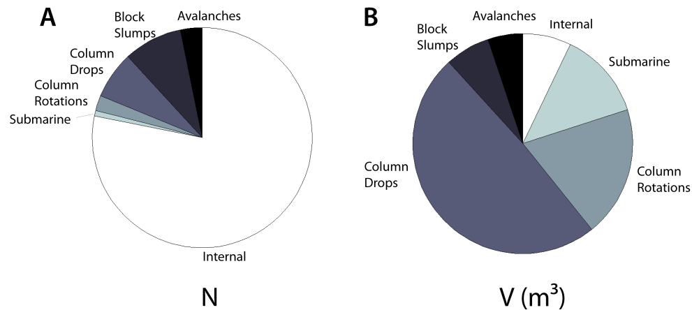
Fig. 1. Distribution of direct calving observations at Kronebreen.
