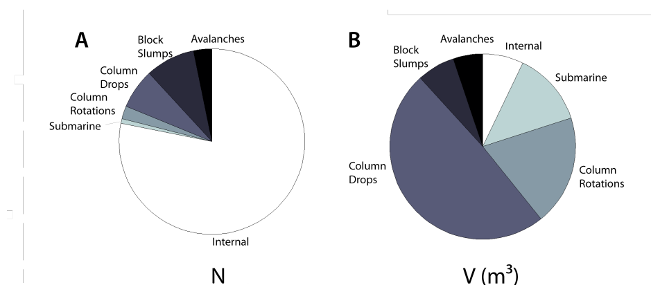
Fig. 1. Distribution of direct calving observations at Kronebreen.
