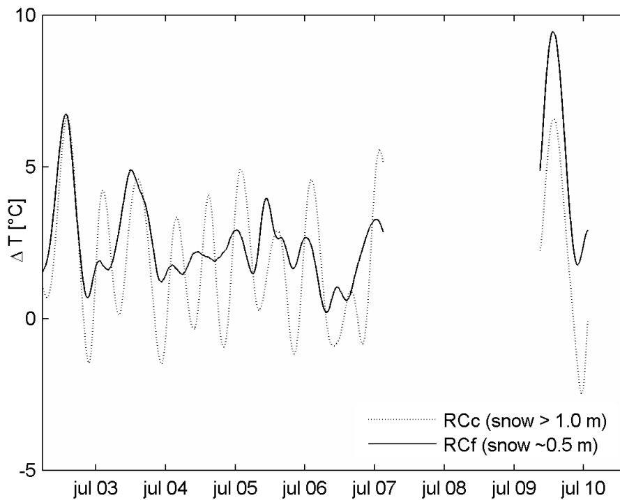
Fig. 2. Temperature differences between ground surface temperature and air temperature for a site with a maximum snow cover of 1m and a site with a thin snow cover of around 0.5 m.
