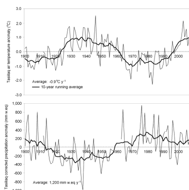
Time series of atmospheric values from Tasilaq meteorological station for 1900–2008: MAAT anomaly and 10-years running average; and annual corrected precipitation anomaly and 10-years running average (this figure is from Mernild et al. 2011, The Holocene).
