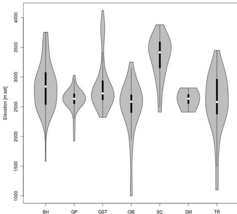
Fig. 3. Elevation range of each type of evidence (except rock glaciers). The plot shown is a combination of a box plot (the white dot is the median, the black boxes range from the lower to upper quartile, and the thin black lines represent the whiskers) and a kernel density plot super-imposed in a mirror image fashion (grey shaded areas).
