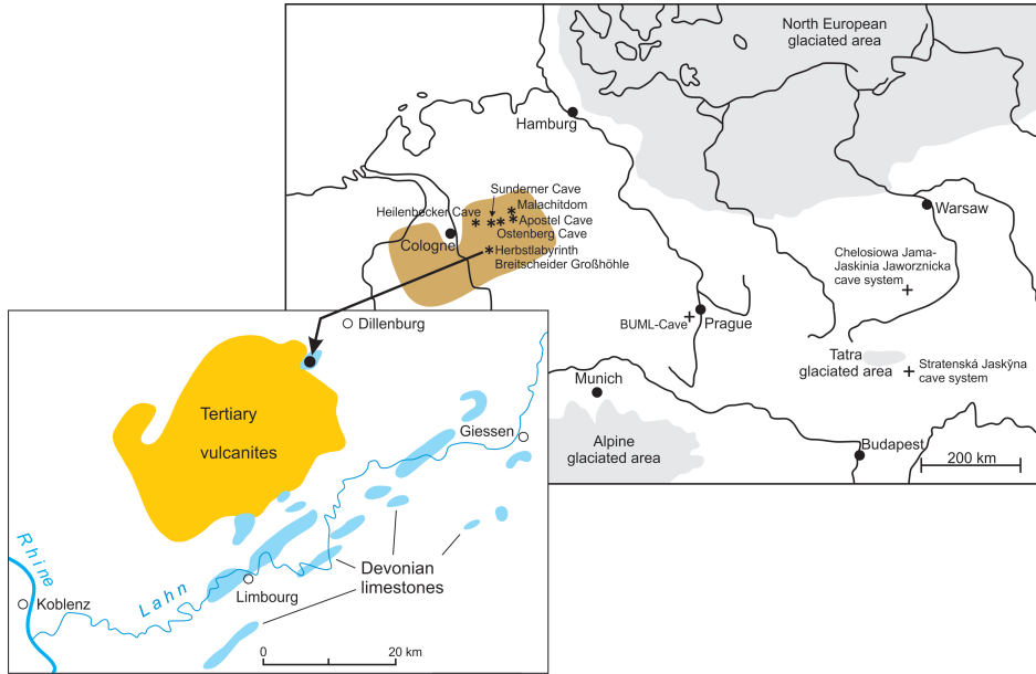
Fig. 1. Map showing the position of the “Herbstlabyrinth-Advent” Cave system as well as the other caves of Central Europe from which cryocalcites have been described (light brown – Rhenish Slate Mountains, li
