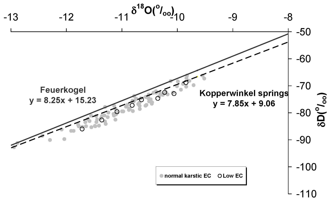
Fig. 3. Figure 4. Stable isotopic characteristics of the Saarhalle ice core and the potential sources. (See full caption in the revised manuscript)
