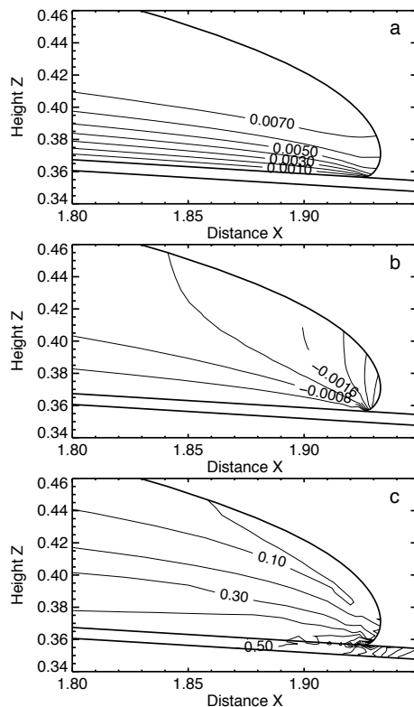
Fig. 8. Experiment A: Relatively stiff and moderately non-linear till ( m=3 , B=8 ): Snapshots at dimensionless time T=15.4 showing the distribution of horizontal velocity (a) , vertical velocity (b) and effective stress (c) in the frontal part of the glacier. Note that the effective stress in the sediment is decreasing distal of the glacier front.
