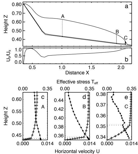
Fig. 10. Experiment B: Relatively soft and moderately non-linear till ( m=3 , B=0.35 ): (c–e) vertical profiles of the non-dimensional horizontal velocity U (lines with crosses) and effective stress T_{\text{eff}} (lines with dots) are shown at a dimensionless time T=15 for the three locations A, B and C shown in (a) . Note that the vertical scale changes for each profile. (b) shows the ratio between the horizontal velocity at the ice-sediment interface U_b to the one at the glacier surface U_s .
