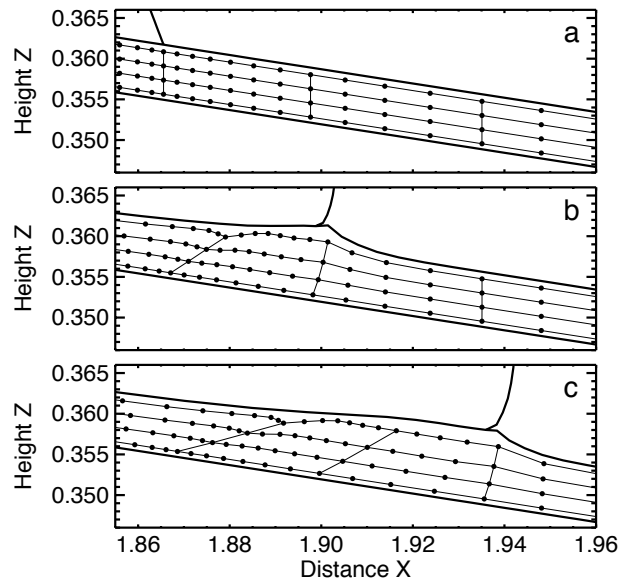
Fig. 12. Experiment C: Moderately stiff and moderately non-linear till ( m=3 , B=0.79 ): Sediment layers which were originally parallel to the bed (a) are deformed and form a wave to keep the sediment bulge in position (b–c) . The snapshots were taken at dimensionless times T equal to 0 (a) , 8 (b) and 14 (c) . Three vertical straight lines in (a) are followed throughout (b–c) .
