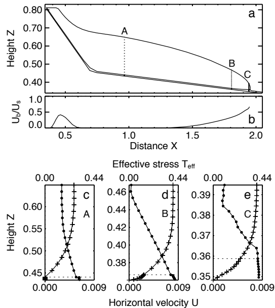
Fig. 14. Moderately stiff and highly non-linear till ( m=40 , B=0.42 ): (c–e) vertical profiles of the horizontal velocity (lines with crosses) and effective stress (lines with dots) are shown at a dimensionless time T=15 for the three locations A, B and C shown in (a). (b) shows the ratio between the horizontal velocity at the ice-sediment interface U_b to the one at the glacier surface U_s .
