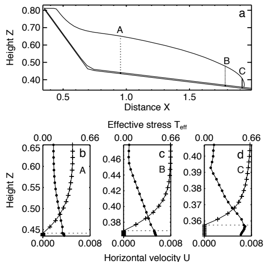
Fig. 3. Experiment A: Relatively stiff and moderately non-linear till ( m=3 , B=8 ): (b–d) vertical profiles of the non-dimensional horizontal velocity U (lines with crosses) and effective stress T_{\text{eff}} (lines with dots) are shown at a dimensionless time T=15.4 for the three locations A, B and C shown in (a) . Note that the vertical scale changes for each profile.
