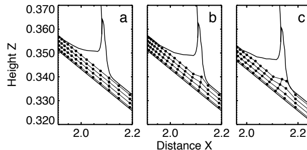
Fig. 6. Experiment B: Relatively soft and moderately non-linear till ( m=3 , B=0.35 ): Three snapshots ( a–c ) at intervals of two dimensionless time units T show the evolution of five internal sediment layers which are parallel at the time T=15 (a), when the sediment bulge had an almost stable slope. Sediment uplift takes place at the transition from the down-facing bulge slope to the undisturbed sediment layer (b–c). A vertical straight line in (a) is followed throughout (b–c).
