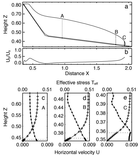
Fig. 13. Experiment C: Moderately stiff and moderately non-linear till ( m=3 , B=0.79 ): (c–e) vertical profiles of the non-dimensional horizontal velocity U (lines with crosses) and effective stress T_{\text{eff}} (lines with dots) are shown at a dimensionless time T=15 for the three locations A, B and C shown in (a) . Note that the vertical scale changes for each profile. (b) shows the ratio between the horizontal velocity at the ice-sediment interface U_b to the one at the glacier surface U_s .
