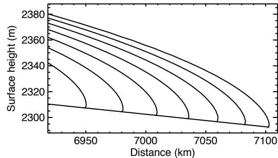
Fig. 15. Glacier advance calculated with a altitude-dependent mass balance distribution over the whole glacier as used in Leysinger Vieli and Gudmundsson (2004) and shown using the same scale as in Fig. 2a.
