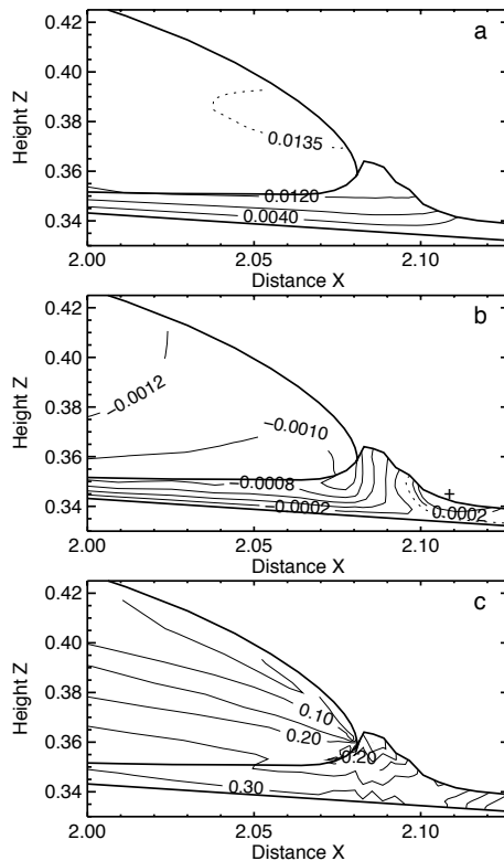
Fig. 7. Experiment B: Relatively soft and moderately non-linear till ( m=3 , B=0.35 ): Snapshots at dimensionless time T=15 showing the distribution of horizontal velocity (a) , vertical velocity (b) and effective stress (c) in the frontal part of the glacier. In (b) the dashed line represents the zero velocity contour line and the symbol + means positive vertical velocities, that is upward movement.
