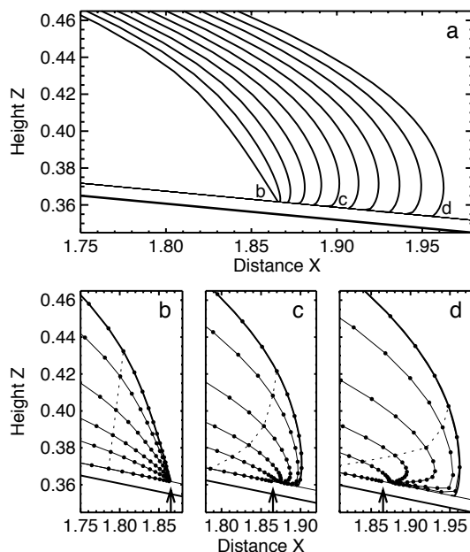
Fig. 2. Experiment A: Relatively stiff and moderately non-linear till ( m=3 , B=8 ): (a) glacier surfaces are shown at time intervals of approximately two dimensionless time units. Selected front positions and surface shapes marked (b) , (c) and (d) are shown in more detail in subfigures (b–d) . (b–d) snapshots of the front showing the surface, four selected internal layers and the ice-sediment interface at dimensionless times T equal to 0 (b) , 10 (c) and 20 (d) . The dots indicate material particles that can be followed throughout the three pictures. The connecting lines illustrate how material layers (fine solid and dashed lines) with initial shape as in (b) become deformed with time. The arrow marks the initial position of the glacier front.
