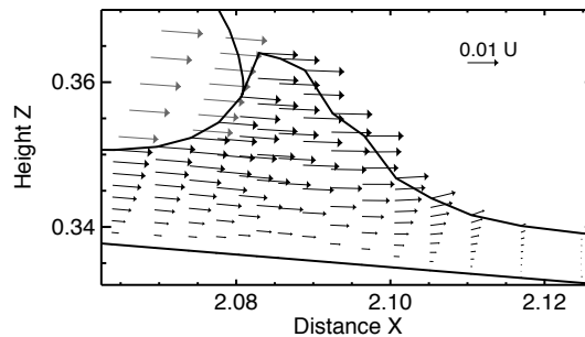
Fig. 9. Experiment B: Relatively soft and moderately non-linear till ( m=3 , B=0.35 ): Velocity vectors of the sediment bulge are shown at the dimensionless time T=15 . Velocity vectors are mostly parallel to the bed. Sediment uplift takes place at the downfacing side of the bulge.
