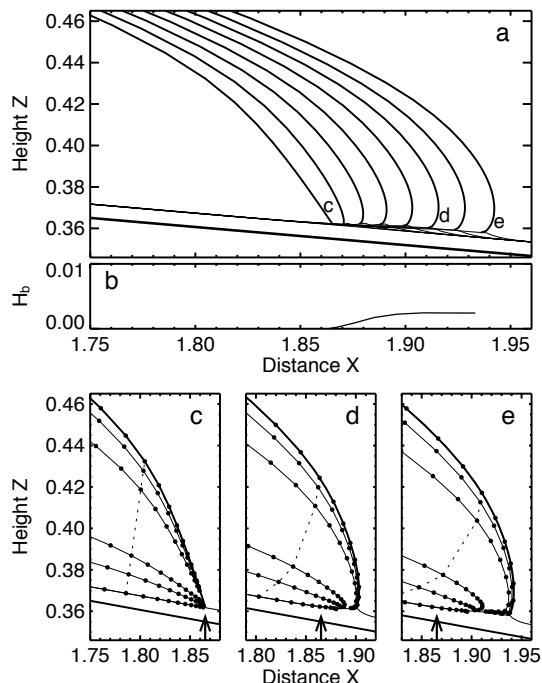
Fig. 11. Experiment C: Moderately stiff and moderately non-linear till ( m=3 , B=0.79 ): (a) glacier surfaces are shown at time intervals of approximately two dimensionless time units. Selected front positions marked c, d and e are shown in more detail in subfigures (c–e). (b) shows the maximum height H_b of the sediment bulge with its horizontal position. Note that the bulge is significantly smaller than in Fig. 4. (c–e) snapshots of the front showing the surface, four selected internal layers and the sediment surface at dimensionless times T equal to 0 (c) , 8 (d) and 14 (e) . The dots indicate material particles that can be followed throughout the three pictures. The connecting lines illustrate how material layers (fine solid and dashed lines) with initial shape as in (c) become deformed with time. The arrow marks the initial position of the glacier front.
