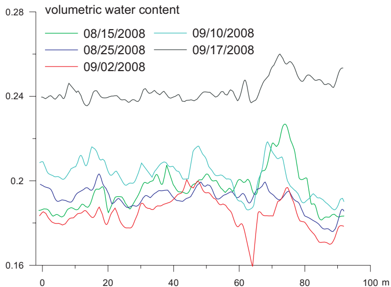
Fig. 7. Transect T1: average volumetric soil water content of the active layer over a distance of 95 m.
