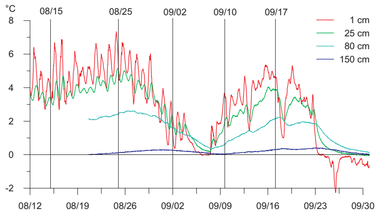
Fig. 6. Temperature profile in the active layer at the position 123.6 m of transect T2. The two lower sensors have been added on 20 August 2009. The dates of the radar surveys of transect T2 are indicated as vertical lines.
