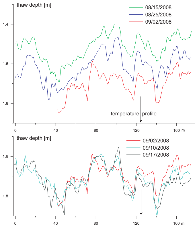
Fig. 5. Transect T2: thaw depth inferred from multi-channel-GPR over a transect length of about 175 m. For unknown reasons, the survey of transect T2 conducted on 2 September yields only a weak and discontinuous reflection to about the 40 m mark, so that it is not possible to infer meaningful thaw depths for this part of the transect. The arrow indicates the position of the instrumented temperature profile (Fig. 6).
