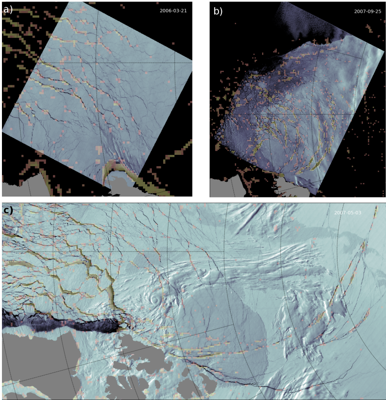
Fig. 5. Comparison of thin ice concentrations with optical satellite images (MODIS band 3). The optical images are displayed in grayscale, TICs are displayed in opaque color from reddish (5%) to yellow (100%). The TIC pixel cover an area of 6.25 km×6.25 km.
