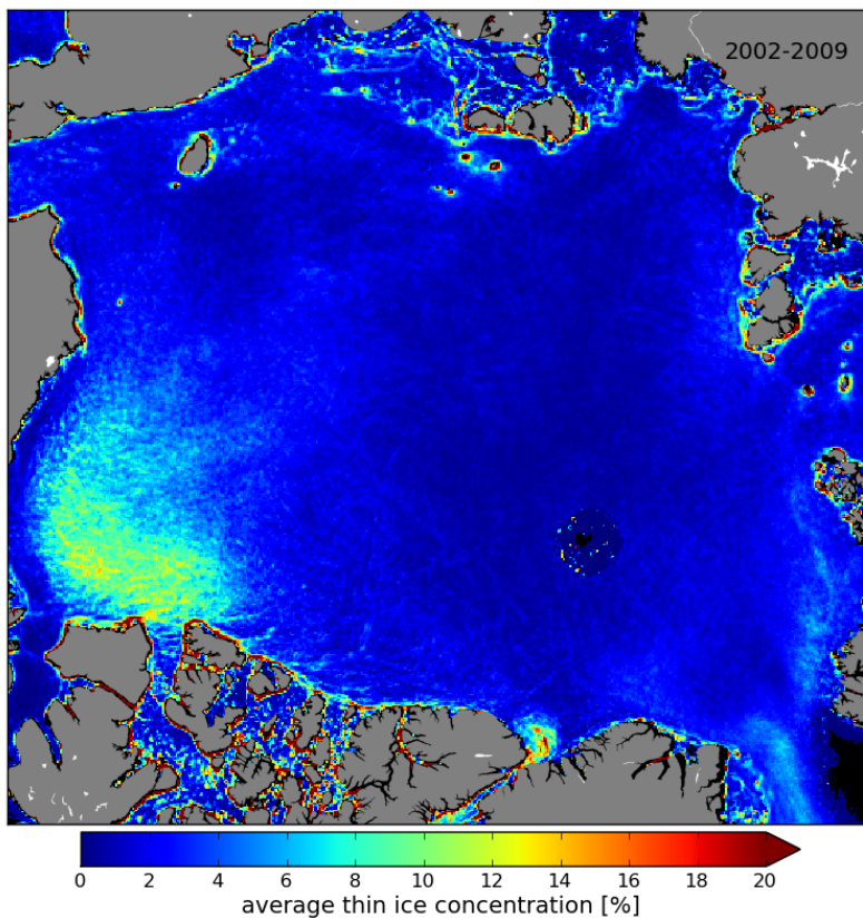
Fig. 6. Average of thin ice concentrations from 2002 to 2009 excluding the summer months June, July and August.
