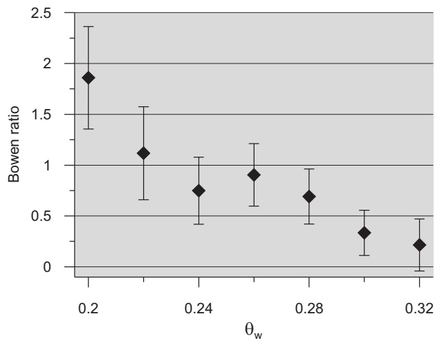
Fig. 4. Average daily Bowen ratio vs. volumetric soil water content \theta_w in soil water content classes of widths of 0.02 for the summer period from 1 Jul to 31 Aug 2008 (see Fig. 3). The points are drawn at the center of each class, and the error bars represent the standard deviation of the Bowen ratio values within one class. Three days with negative average Q_h are discarded.
