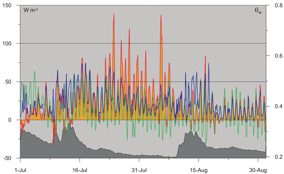
Fig. 3. Sensible (red), latent (blue) and ground heat fluxes (green) for the summer period from 1 Jul to 31 Aug 2008 (left axis). The soil water content \theta_w measured with Time Domain Reflectometry at a depth of 0.1 m at the Bayelva climate station is shown below (right axis).
