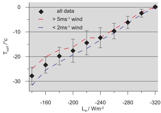
Fig. 7. Surface temperature T_{surf} vs. incoming long-wave radiation L_{in} during the dark winter period in classes of L_{in} of 20 Wm^{-2} width. The points are drawn at the center of each class, and the error bars represent the standard deviation of the surface temperature values within one class. The red and blue lines represent the average curves for situations with high and low wind speeds.
