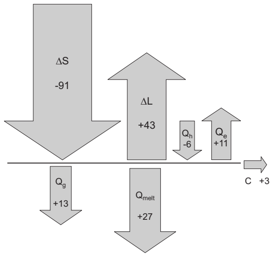
Fig. 12. Schematic diagram of the contributions of the surface energy budget for the snow melt period. Notation as in Fig. 2
