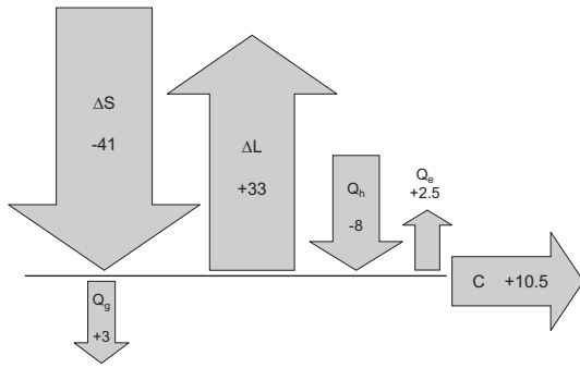
Fig. 11. Schematic diagram of the contributions of the surface energy budget for the pre-melt period. Notation as in Fig. 2
