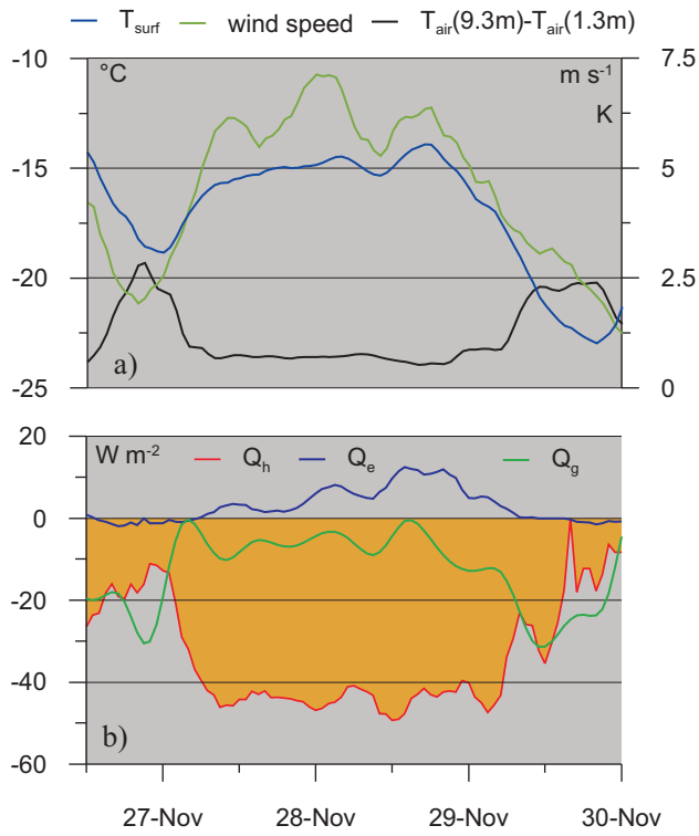
Fig. 8. a) Surface temperature (left axis), wind speed (right axis), and temperature difference at the gradient tower (right axis) for a period in November 2008. The snow depth was 0.7 m at this time. b) Sensible heat flux Q_h , latent heat flux Q_e and snow heat flux Q_g (conduction method) for the same period.
