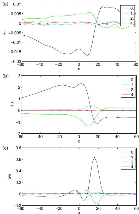
Fig. 7. Residuals \Delta d_i between observations and FE-model predictions for (a) surface topography, (b) horizontal and (c) vertical velocity. The dotted lines correspond to the square-roots of the main diagonal of the data covariance matrix \mathbf{C}_D determined with the optimal interpolation method BLUE.
