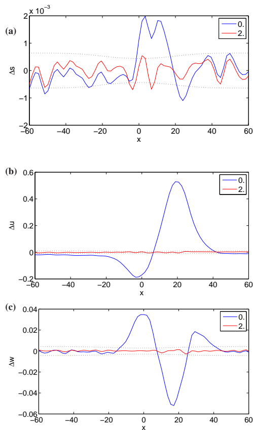
Fig. 5. Residuals between observations and FE-model predictions for (a) surface topography, (b) horizontal and (c) vertical velocity. The residuals are defined as \Delta \mathbf{d}_i = \mathbf{d} - \mathbf{g}(\mathbf{m}_i) with i the iteration number. The dotted lines correspond to the square-roots of the main diagonal of the data covariance matrix \mathbf{C}_D determined with the optimal interpolation method BLUE. Note that the first and second iteration lines are almost superimposed in panel (a).
