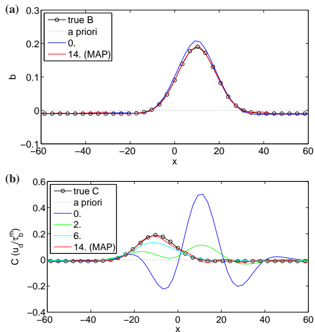
Fig. 10. Inferred (a) bed topography and (b) basal slipperiness distributions for non-linear ice rheology and non-linear sliding law with basal sliding exponent m=3 and basal perturbation amplitudes of 0.2.
