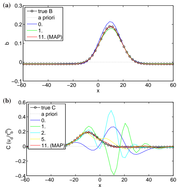
Fig. 8. Inferred (a) bed topography and (b) basal slipperiness distributions for non-linear rheology and perturbation amplitudes of 0.2. \alpha=0.2^\circ , \bar{C}=200 , n=3 and \tau_0=0.3 . Note superimposing of MAP line with true bedrock topography in panel (a).
