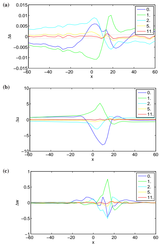
Fig. 9. Residuals between observations and FE-model predictions for (a) surface topography, (b) horizontal and (c) vertical velocity. The dotted lines correspond to the square-roots of the main diagonal of the data covariance matrix C_D .
