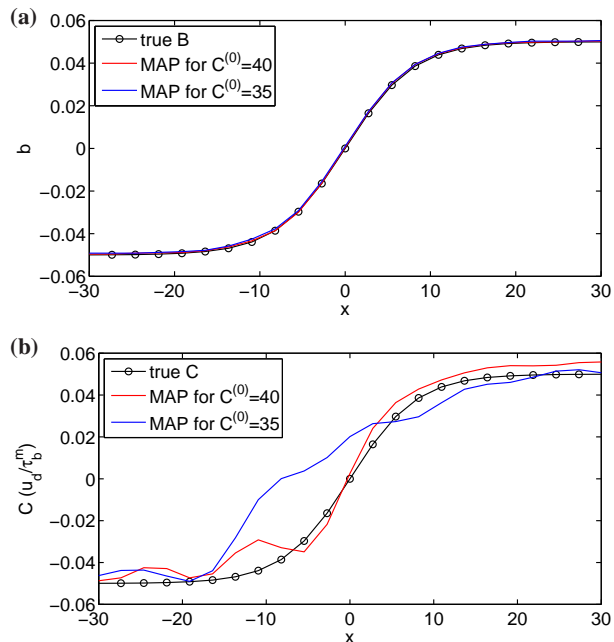
Fig. 14. Comparison between MAP (a) bed topography and (b) basal slipperiness as obtained with the true model characteristics ( u_d=1.27 \text{ m a}^{-1} , \bar{C}=40 ; red lines) and with the wrong estimated model characteristics ( u_d=1.45 \text{ m a}^{-1} , \bar{C}=35 ; blue lines). The true basal perturbations are also shown for comparison (black lines with circles).
