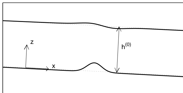
Fig. 1. Illustration of the problem geometry and coordinate system. Gaussian-shape bedrock perturbation and corresponding surface reaction are shown as a black line. The dashed lines show the undisturbed glacier geometry.
