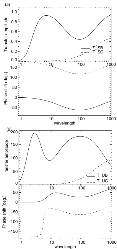
Fig. 2. (a) Steady-state amplitude ratios and phase shifts for both bedrock ( T_{sb} ) and basal slipperiness perturbations ( T_{sc} ). (b) Steady-state amplitude ratios and phase shifts of surface-parallel velocities for a bedrock ( T_{ub} ) and basal slipperiness perturbation ( T_{uc} ). The medium is Newtonian. The mean surface slope is 0.5^\circ and the mean non-dimensional basal slipperiness is \bar{C}=200 .
