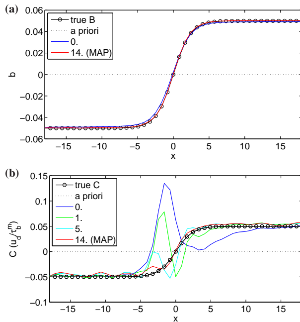
Fig. 12. Inferred (a) bed topography and (b) basal slipperiness distributions for a temperature dependent ice rheology ( n=3 , \tau_0=0 ). The temperature varies linearly across the ice depth from -25^\circ at the surface to 0^\circ at the bottom.
