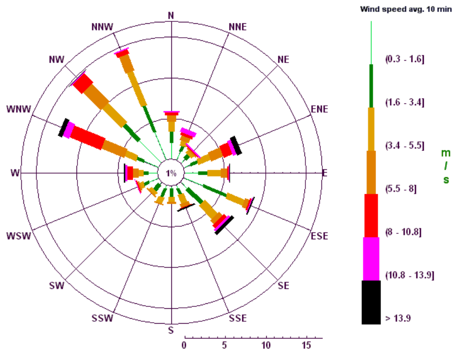
Fig. 5. Rose diagram showing wind direction (deg.) and speed (m/s) from August 2007 to August 2008 at Ripfjorden Weather Station (source: http://158.39.11.101/command=RTMC&screen=WindYear%20%20 ).
