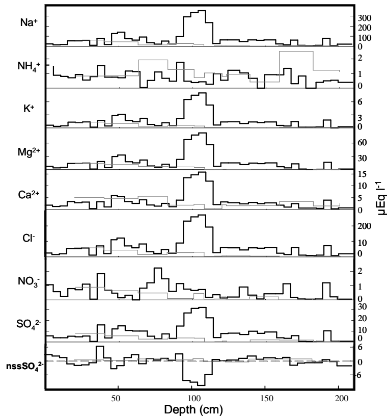
Fig. 3. Ion concentration (in \mu\text{Eq l}^{-1} ) in Pit 1 (black histogram) and Pit 2 (grey histogram).
