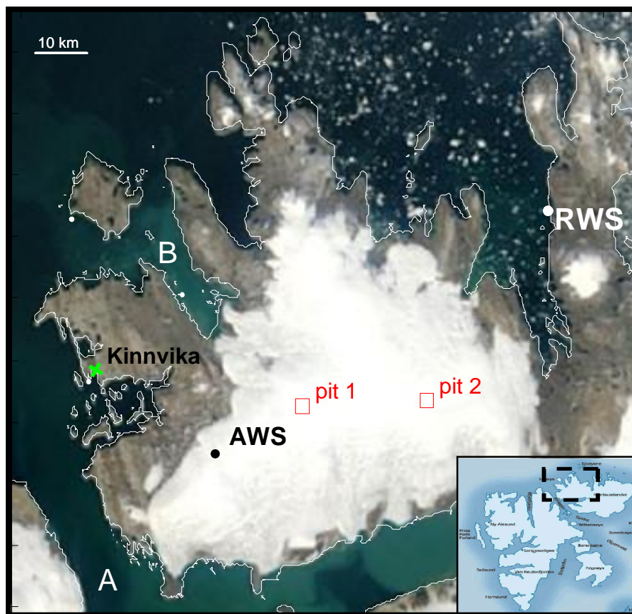
Fig. 1. Satellite image (image from NASA) of western Nordaustlandet with location of Kinnvika station, snow-pit sampling sites (Pit 1 and Pit 2), Automatic Weather Station (AWS), Ripfjorden Weather Station (RWS), Hinlopen straight (A) and Lady Franklinfjorden (B).
