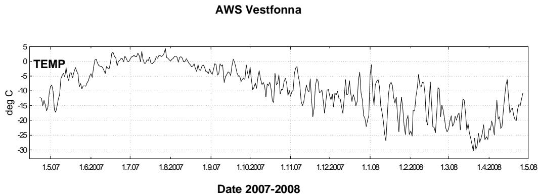
Fig. 4. Temperature ( ^{\circ}\text{C} ) plotted from AWS (R. Hock and U. Jonsell, personal communication, 2008).
