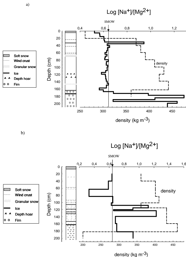
Fig. 2. Stratigraphy and depth profile of the melting indicator \text{Log} [\text{Na}^+]/[\text{Mg}^{2+}] in \mu\text{Eq l}^{-1} (solid line) and density (dashed line) for (a) Pit 1 and (b) Pit 2. The black arrow points the melting indicator value for Standard Mean Ocean (SMOW).
