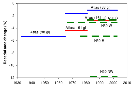
Fig. 11. Decadal area changes calculated for the inventory sample of 38 glaciers since the 1930s (blue line), the inventory sample of 161 glaciers since Atlas69 (red line) and the N50 sample (green dashed line) divided into W: West, C: Central, E: Eastern and NW: NorthWest (see Table 1).
