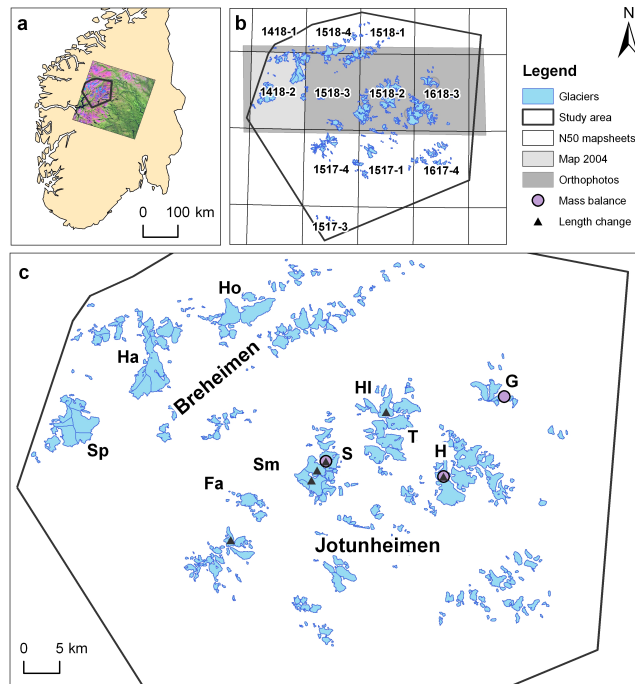
Fig. 1. (a) Location map of southern Norway with a false colour composite of bands 543 (as RGB) of the Landsat TM scene (199–17) and extent of study area. (b) The N50 map sheets and glaciers in the study area. (c) Glaciers (>0.01 km 2 ) in the Breheimen and Jotunheimen region. Letter codes denote: Sp: Spørteggbreen, Ha: Harbardsbreen, Ho: Holåbreen, Fa: Fanaråken, Sm: Smørstabbreen, S: Storbreen, HI: Heimre Illåbreen, T: Tverråbreen, H: Hellstugubreen, G: Gråsubreen.
