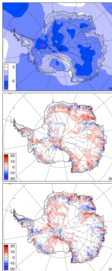
Fig. 11. Summer averages of (a) ABL mean potential temperature deficit in K, (b) AdvV in K per day and (c) AdvH in K per day.
