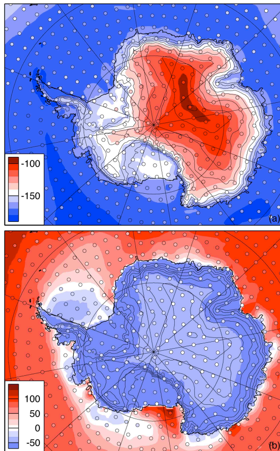
Fig. 3. Comparison of observed (circles, Zhang et al., 2004) and simulated TOA net radiative emission ( \text{W}/\text{m}^2 ) for 1983 to 2004, for (a) Winter (JJA) and (b) Summer (DJ). Positive values indicate net fluxes into the atmosphere.
