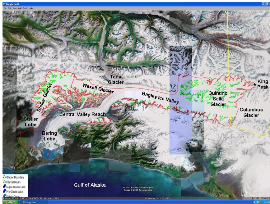
Fig. 2. Bering Glacier System, Alaska. Glacier outlines digitized in GLIMSVIEW displayed in Google Earth™. The Surging Bering Glacier (SBG) and Steller Glacier are outlined in red. Together the SBG and Steller Glacier comprise the complete Bering Glacier System – as is recognized by the U.S. Board on Geographic Names. Nunataks are outlined in light green and debris covered areas are outlined in dark green.
