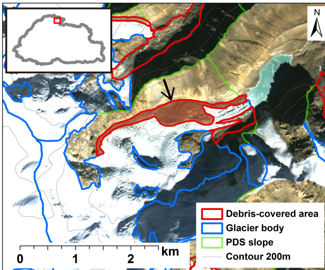
Figure S1. Example of irregularly supplied debris cover (shading), probably supplied from the neighbouring PDS-slope (allow). Inset figure shows the location.
