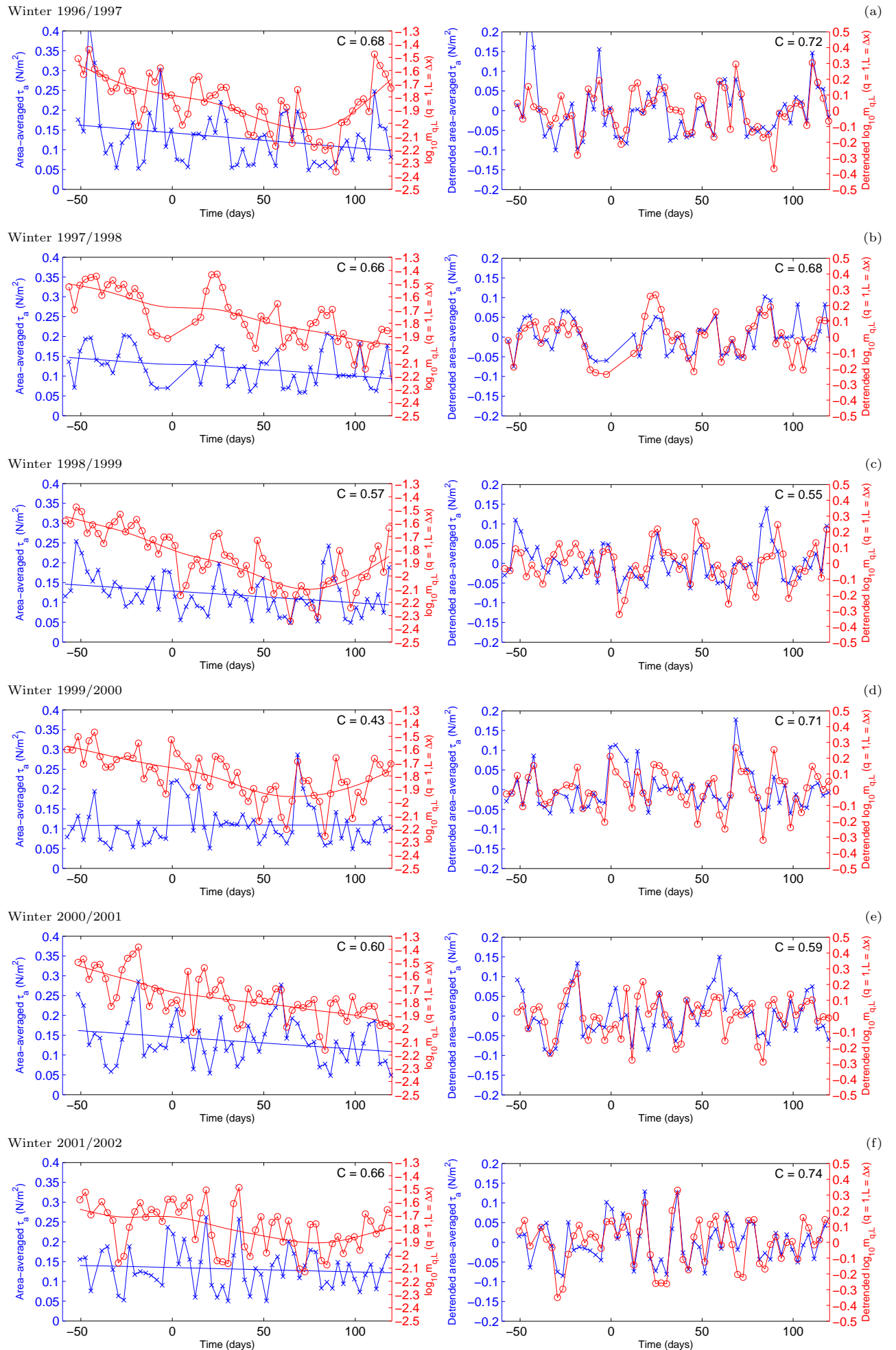
Supplementary Figure 1. Time series of \bar{\tau}_a ( N/m^2 ) and \bar{m}_{q,L} (for q = 1 and L = \Delta x ) in the 11 analyzed winter seasons (a–k): original data with trend lines (left) and detrended data (right). Time is shown in days after 1. January of the respective year.
