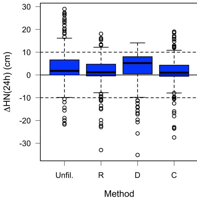
Fig. 5. Difference between measured and simulated 24-h new snow amounts \Delta\text{HN}(24\text{h}) for the winter 2009–2010 at Mt. Fidelity Study Plot. Shown are the differences for the simulation with unfiltered (Unfil.) and filtered precipitations amounts using ratio method (R), difference method (D) and constant method (C). Boxes, whiskers and open circles as in Fig. 2. Dashed lines are located at \pm 10 cm.
