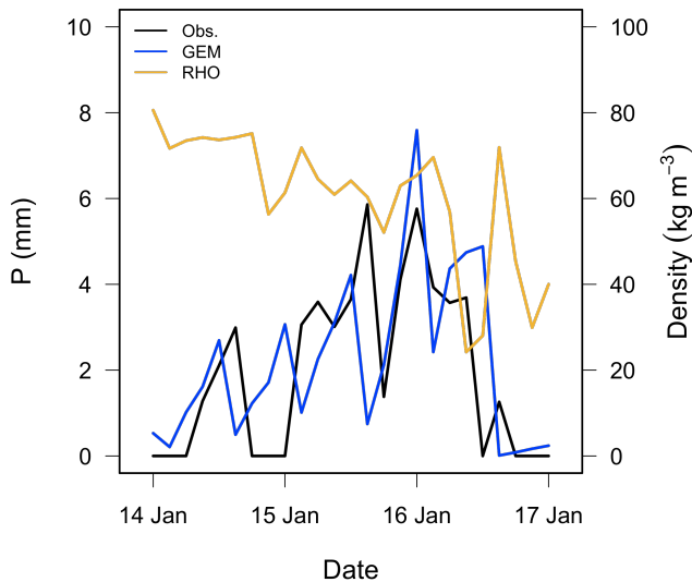
Fig. 10. Observed (Obs.) and forecasted (GEM) 3-hourly precipitation amounts as well as the modeled initial new snow density (RHO) for the period of 14 to 16 January 2010 at Mt. Fidelity Study Plot. Values located at the tick marks correspond to the midnight values.
