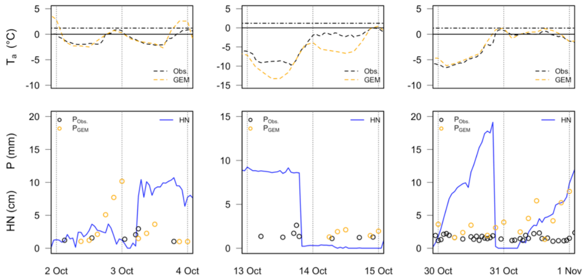
Fig. 9. Comparison of observed (Obs.) and forecasted (GEM) parameters for three precipitation events during October 2009 at Mt. Fidelity Study Plot. Upper graphs show a comparison of observed (Obs.) and forecasted (GEM) air temperature during these three events (same time scale as lower graphs). Horizontal dash-dotted line indicates the static 1.2 °C threshold used by SNOWPACK to distinguish between snow and rain. Lower graphs show the measured hourly precipitation amounts (black open circles, P > 1 mm) and the forecasted 3-hourly precipitation amounts (orange open circles, P > 1 mm) as well as the measured new snow amounts (blue solid line).
