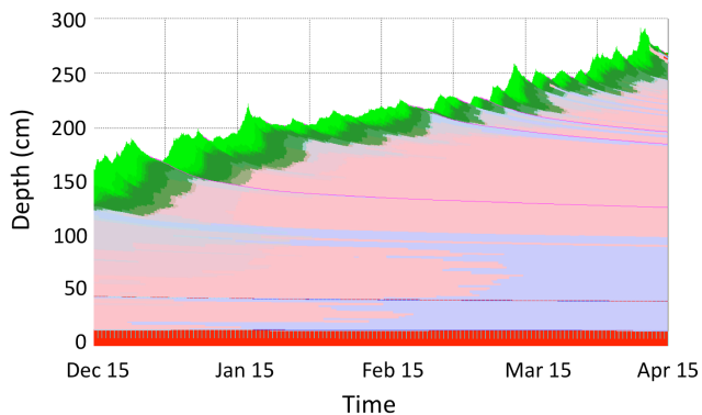
Fig. 7. Snow cover simulation with the snow cover model SNOWPACK for the winter 2009–2010 at Mt. Fidelity Study Plot, Rogers Pass, BC, Canada. Colors represent different grain types (green: precipitation, particles, light pink: rounded grains, blue: faceted crystals, red: melt forms). Purple lines indicate surface hoar layers and hatched layers melt-freeze crusts (upper base and at 50 cm).
