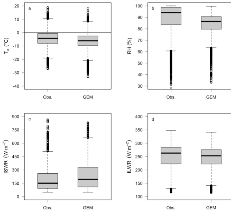
Fig. 6. Comparison of important forecasted (GEM) and observed (Obs.) meteorological parameters. Shown are (a) air temperature ( ^{\circ}\text{C} ), (b) relative humidity (%), (c) incoming short wave radiation ( \text{W m}^{-2} ) and (d) incoming long wave radiation ( \text{W m}^{-2} ) for five winters between 2005 and 2010. For better comparison the incoming short wave radiation only shows values larger than 50 \text{ W m}^{-2} .
