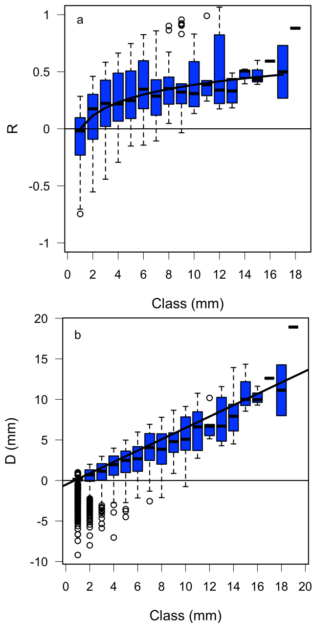
Fig. 2. Correction factors per precipitation class for (a) R (Eq. 1), and (b) D (Eq. 2). Solid lines show a logarithmic fit ( R ) and a linear fit ( D ). The median R^* calculated by Eq. (1) over four winters was 0.12 or 1.32, respectively (compare Eq. 5). Boxes span the interquartile range. Whiskers extend to 1.5 times the interquartile range. Open circles indicate outliers.
