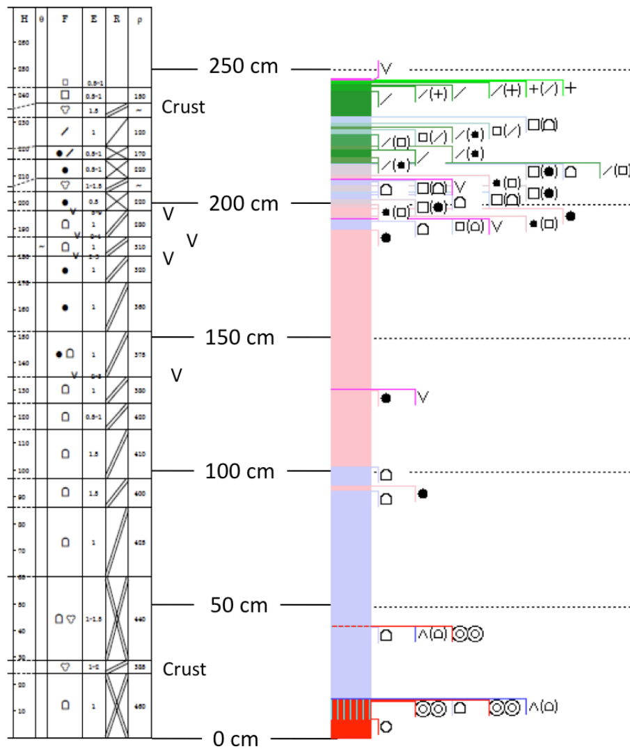
Fig. 8. Observed manual flat field profile (left) and simulated profile (right) for 20 March 2010 at Mt. Fidelity Study Plot. Snow symbols according to Fierz et al. (2009).
