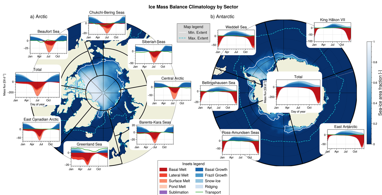
Figure 3. Climatological seasonal cycle of ice mass fluxes for total hemisphere and regional sectors, for Arctic (a) and Antarctic (b). Background maps show the climatological (1979–2008) average sea ice concentration during month of minimum extent (colours), minimum sea ice edge (white solid line) and maximum sea ice edge (cyan dashed line). Each panel provides the climatological seasonal cycle of ice mass fluxes as a function of the day of year, with each coloured area corresponding to a flux (see legend for details), for each sector delimited by the black boundaries on the map; the scales of the y-axes differ among panels but the labels and units are the same (Mass flux, \text{Gt d}^{-1} ). The ice mass transport is shown by a green line, as it can be both positive (ice import) and negative (ice export). The “Total” panels (left for Arctic, centre for Antarctic) show the climatological seasonal cycle for the whole hemisphere.
