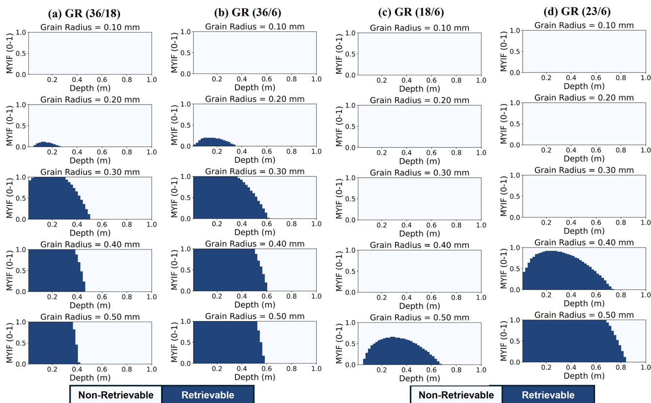
Figure 9. Retrieval of snow depth with GR(36/18), GR(36/6), GR(18/6) and GR(23/6) on different MYIF and grain radius. The corresponding 3D TB plots can be found in the Supplement.
