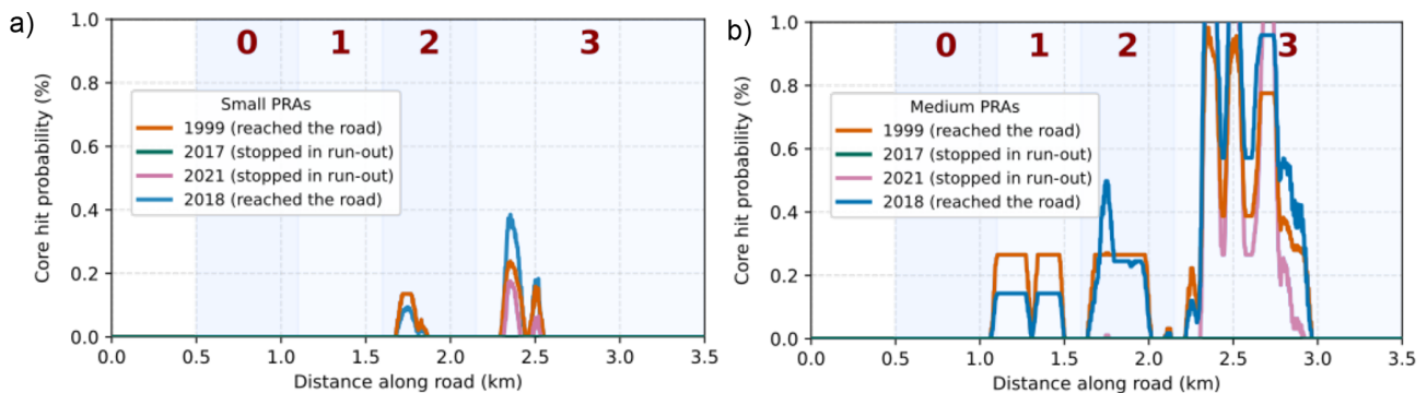
Figure 11. Probability along the road below Brämabüel for small and medium release zones for the events in 1999, 2017, 2018 and 2021. For the events in 1999 and 2018, avalanche paths 1 and 2 reached the road, whereas in 2017 and 2021 the avalanches stopped within the flatter runout zone.
