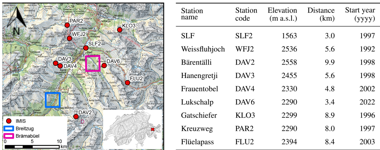
Figure 2. Overview of the IMIS station distribution in the Davos region and the test regions. The table shows the horizontal distances from the stations to the release zone at Brämabüel (map source: Federal Office of Topography).
