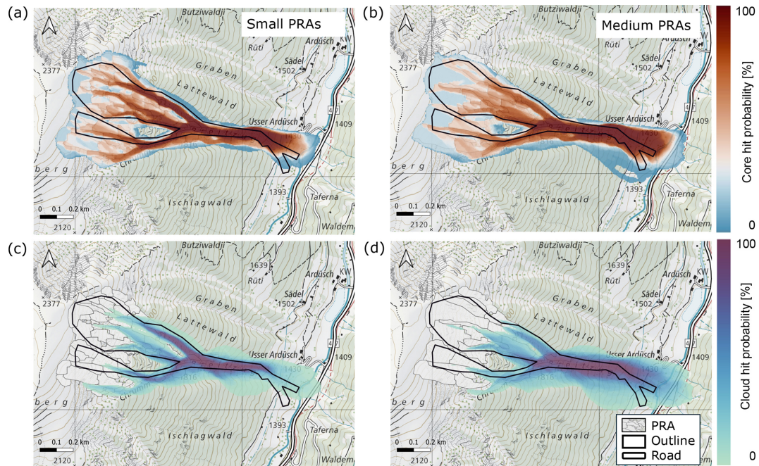
Figure 10. Probability indication map at Breitzug based on the stability approach that includes the stability index and steepness of every single release zone. The PRAs are shown in the background to improve the visibility of the probability indication map in the upper part of the avalanche path (map source: Federal Office of Topography).
