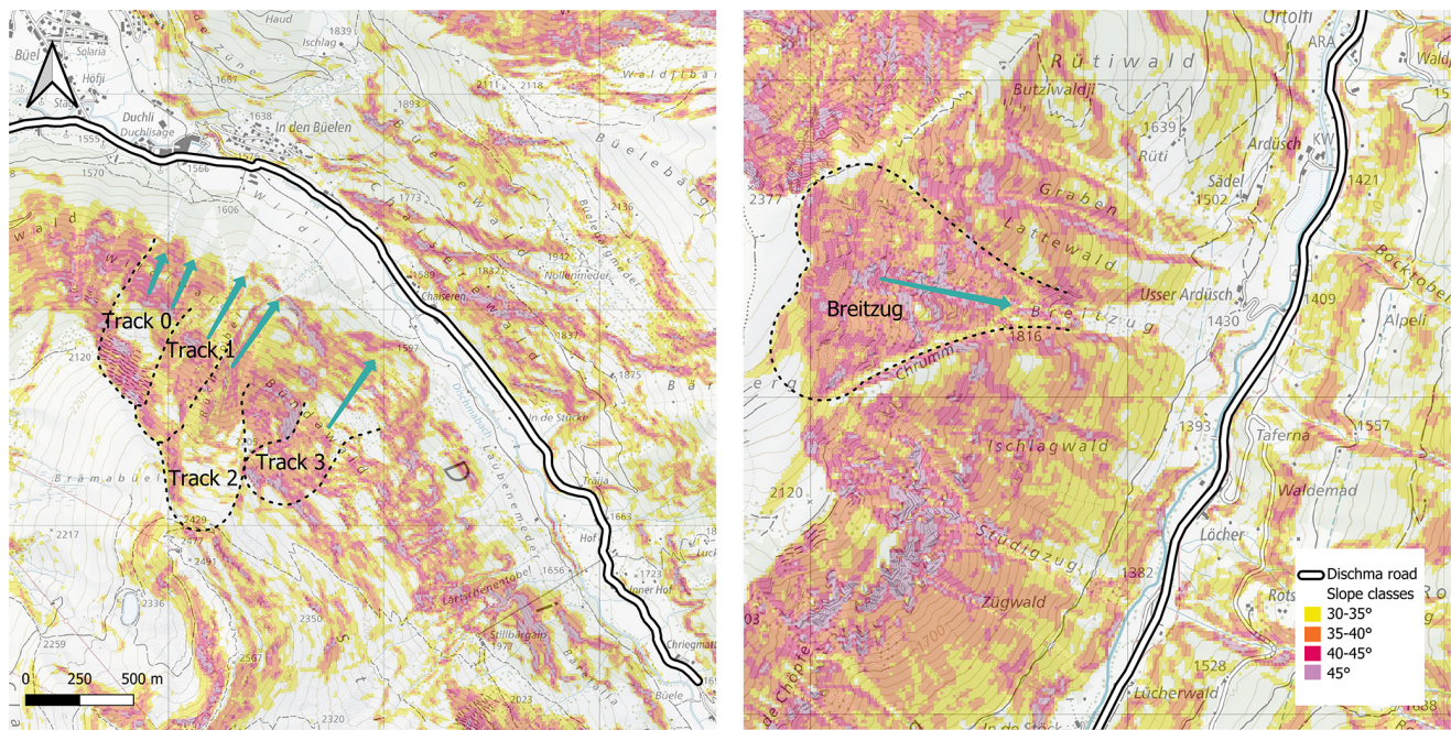
Figure A1. Representation of the Brämabüel and Breitzug avalanche tracks with the slope steepness. For every avalanche track, the main flow direction is indicated by the turquoise arrows (map source: Federal Office of Topography).
