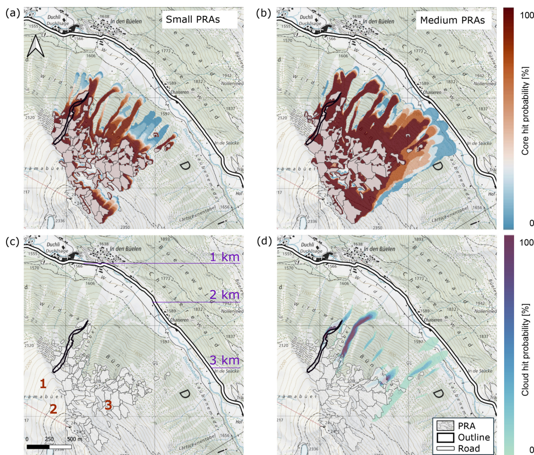
Figure 9. Probability indication map for Brämabüel based on the frequency approach. It is calculated based on snow measurements at all IMIS stations in the region of Davos and the weather forecast of the day before the event on 28 January 2025 12:00 CET. In black, the avalanche outlines are marked for the event that occurred on the morning of 29 January 2025, at 08:00 CET. The avalanche paths 1, 2 and 3 are marked in panel (c) (map source: Federal Office of Topography).
