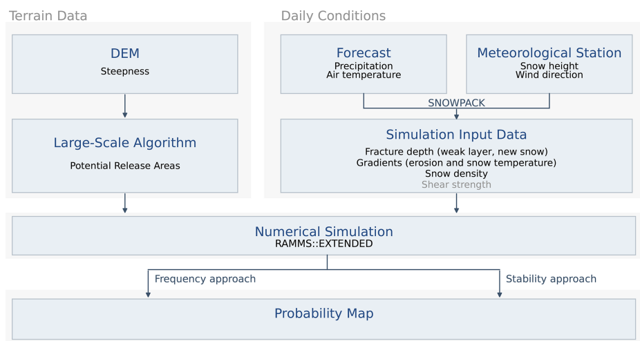
Figure 4. Conceptual presentation of the data flow to produce a probability map. Greyed out are the parameters which are only needed for the stability approach. The detailed inputs used for the SNOWPACK simulations from the meteorological stations are described in Sect. S1 in the Supplement.
