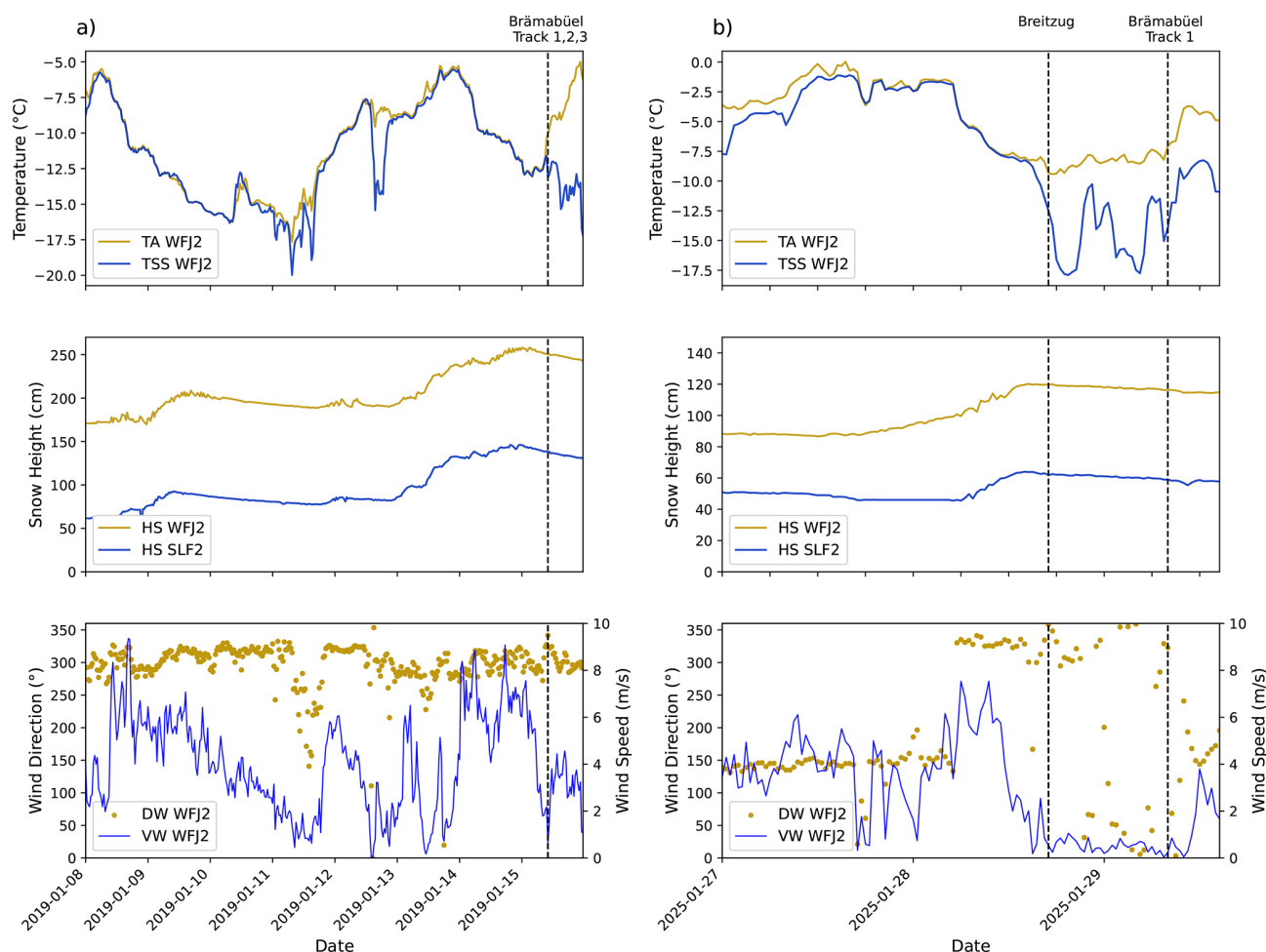
Figure 5. Time series of meteorological observations recorded at the Weissfluhjoch (WFJ2) and Davos valley (SLF2) IMIS stations during the snowfall events preceding the evaluated avalanche releases. Shown are air temperature (TA), snow surface temperature (TSS), total snow height (HS), wind direction (DW), and wind speed (VW). The timing of avalanche release and name of the track is indicated by vertical bars. Columns (a) and (b) correspond to the snowfall periods in 2019 and 2025, respectively. Data source: IMIS.
