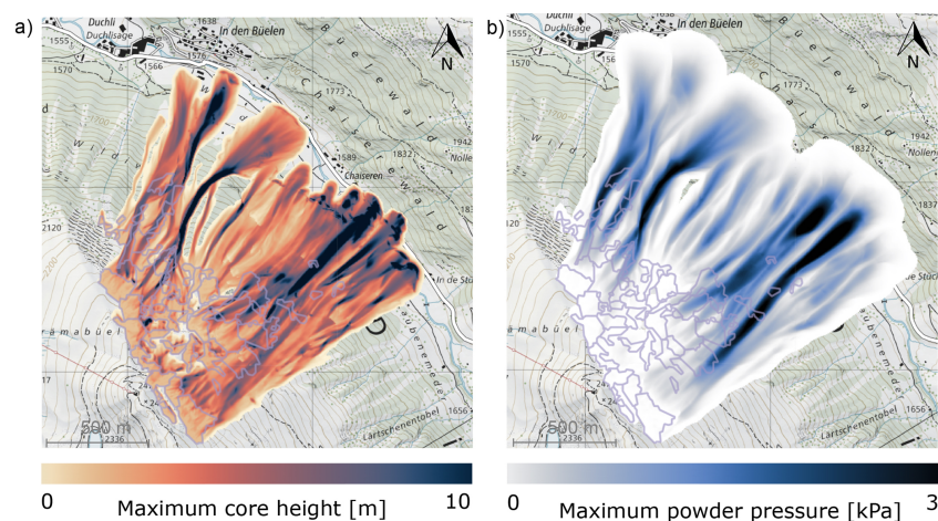
Figure 6. Example of the calculation results of the maximum core height and powder pressure for medium-sized release zones with an expected new snow depth of 1.6 m in the flat field for the Brämabüel test site (map source: Federal Office of Topography).
