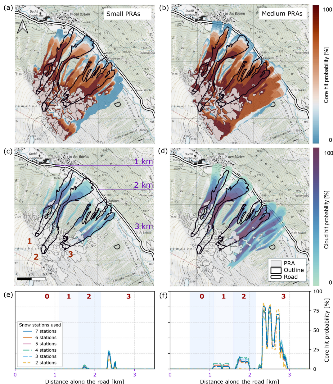
Figure 7. Resulting probability indication maps for the Brämabüel test site based on the frequency approach for small (a, c, e) and medium (b, d, f) release zones based on snow measurements from selected IMIS stations in the Davos region and weather forecasts one day before the event (14 January 2019, 12:00 CET). Black outlines indicate the avalanche event of 15 January 2019. The bottom row shows the calculated hit intensities along the road, based on seven IMIS stations, with stations removed sequentially starting from the farthest one (map source: Federal Office of Topography).
