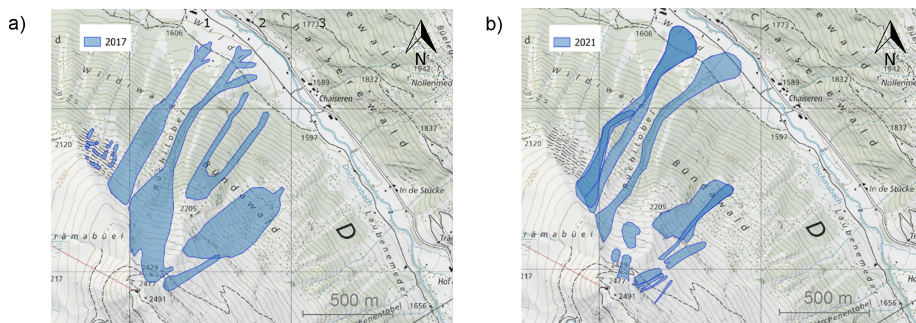
Figure C1. Manually delineated avalanche outlines at Brämabüel for the events of 10 March 2017 (a) and 15 January 2021 (b). For both events, avalanche paths 1 and 2 propagated further downslope than avalanche path 3. For both events, additional avalanche activity is visible within the study area (map source: Federal Office of Topography).
