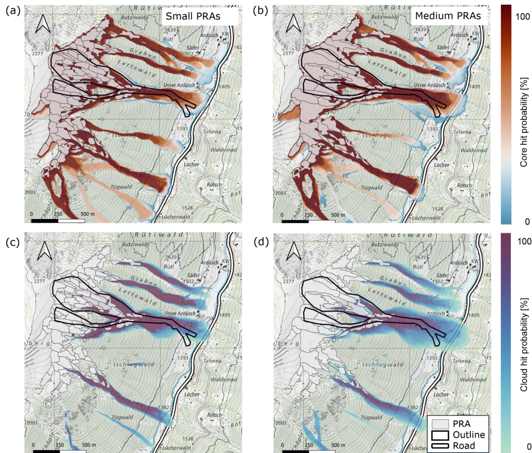
Figure 8. Probability indication map at Breitzug based on the frequency approach issued on 28 January 2025 at 12:00 CET. The avalanche outlines (shown in black) correspond to the event triggered at approximately 17:00 CET on the same day by a Wyssen tower (map source: Federal Office of Topography).
