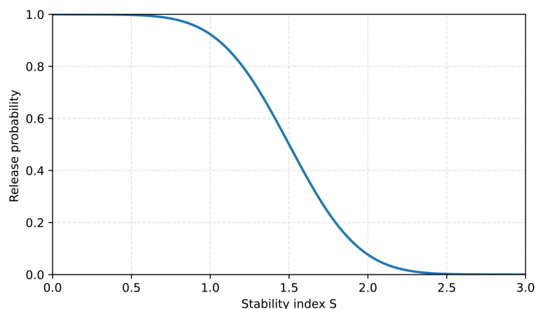
Figure B1. Mapping between the natural stability index S_n and the release probability using the ERF function.
