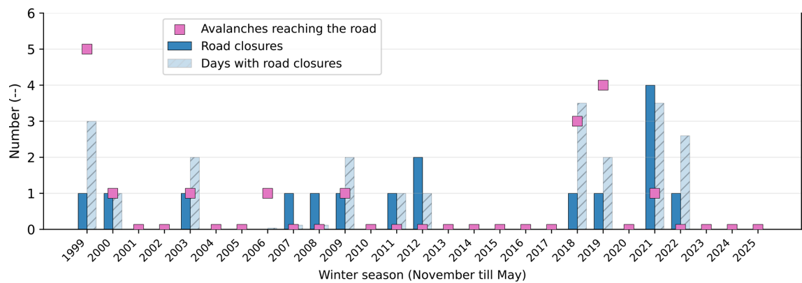
Figure 1. Overview of documented avalanche activity and road closures along the Dischma Valley over the last 26 winter seasons (1999–2025). The analysis is qualitative, as the documentation of avalanche events strongly depends on the availability and quality of the underlying database, which has improved over time. The number of closure days is included to indicate the overall duration and therefore the relative significance of individual road-closure events.
