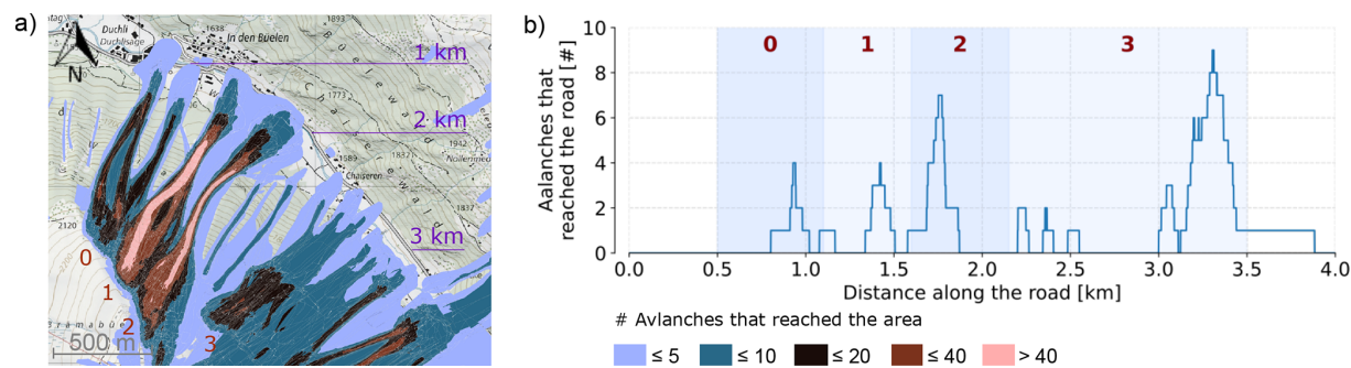
Figure 3. Overview of the mapped avalanche activity affecting the Dischma road near Brämabüel between 1999 and 2025. (a) Number of observed avalanches reaching a pixel. (b) Number of observed avalanches intersecting the Dischma road, shown as distance along the road. The labels 0–3 indicate the main avalanche path sections, and the distance markers in panel (a) correspond to the distance axis in panel (b) . Map source: Federal Office of Topography.
