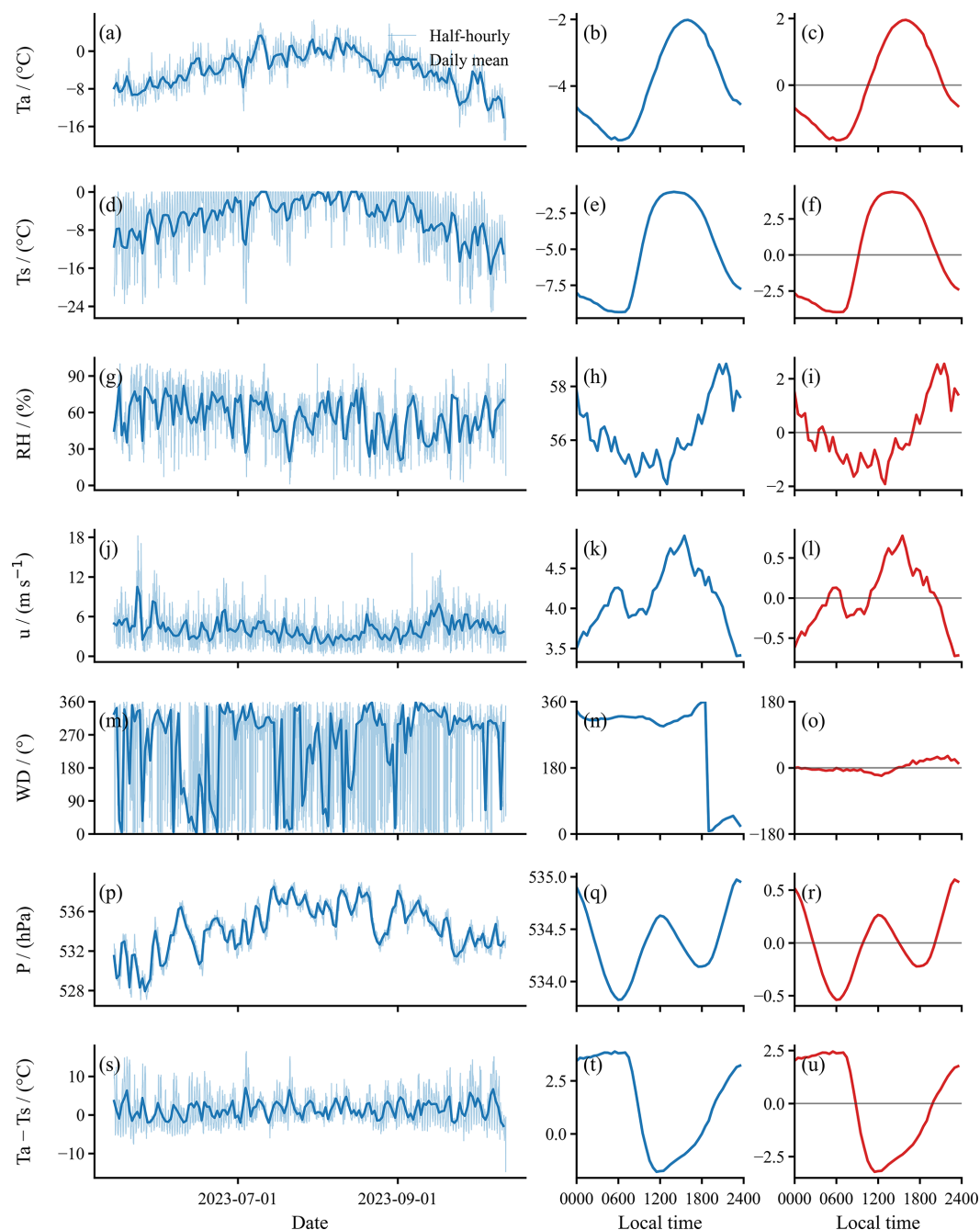
Figure 2. Half-hourly and daily average values (left panels), original mean diurnal cycles (middle panels), and detrended mean diurnal cycles (right panels) of six meteorological variables at the Dundee Glacier for the period May–October 2023: (a–c) air temperature ( T_a ); (d–f) surface temperature ( T_s ); (g–i) relative humidity (RH); (j–l) wind speed ( u ); (m–o) wind direction (WD); (p–r) atmospheric pressure ( P ); and (s–u) surface temperature deficit ( T_a - T_s ).
