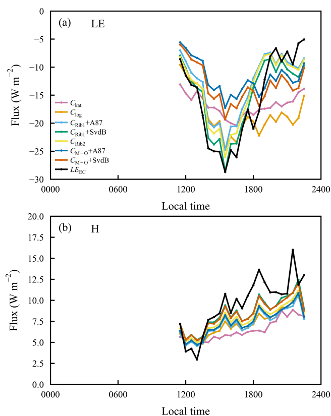
Figure 6. Mean daily cycles of modeled latent heat and sensible heat fluxes obtained from the five different schemes ( C_{kat} , C_{log} , C_{Rib1} , C_{Rib2} , and C_{M-O} ) compared with eddy covariance-derived values ( LE_{EC} and H_{EC} ).
