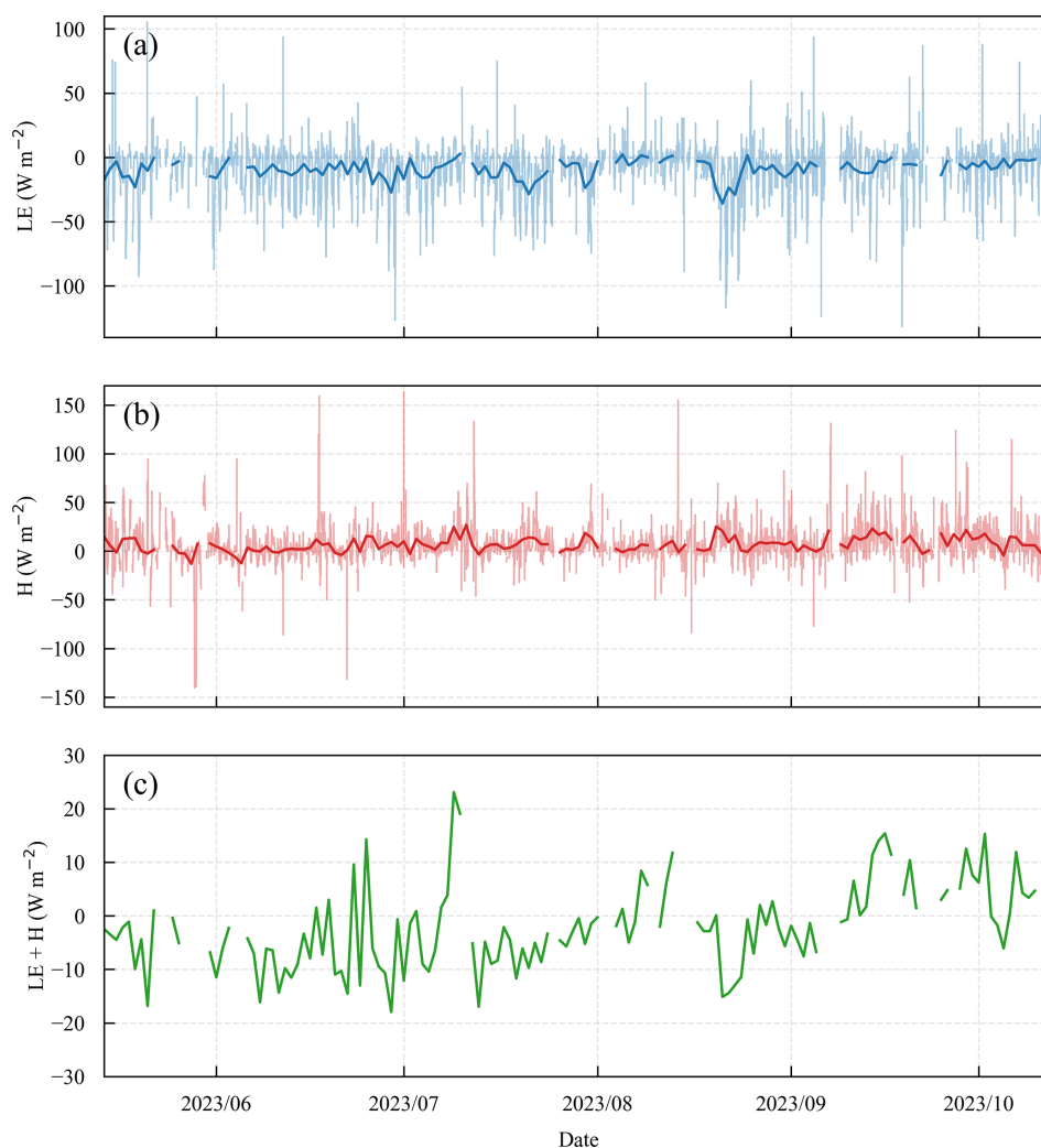
Figure 3. Half-hourly (thin lines) and daily average (thick lines) variations in (a) latent heat flux, (b) sensible heat flux, and (c) total turbulent flux over the Dundee Glacier during the study period. The green line in panel (c) represents the daily average of total turbulent flux.
