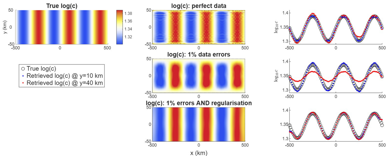
Figure 5. Examples of the basal slipperiness retrieval in \dot{U}a for the same experiment as in Fig. 4. for the laterally-confined channel, for a range of data errors and regularisation parameters of either zero or ( \gamma_a = 1 , \gamma_s = 10^3 \bar{h} ). We show contour plots of the retrieved field in the two-dimensional domain, and also cut-throughs at y = 0.2W and y = 0.8W .
