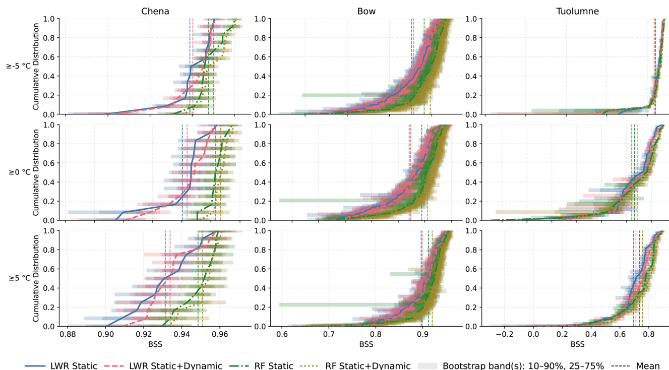
Figure 11. Brier Skill Scores (BSSs) with bootstrap resampling for select temperature thresholds. The CDFs of BSSs show the relative performance of each method compared to the climatology mean. Similar to Fig. 10 but for select temperature thresholds.
