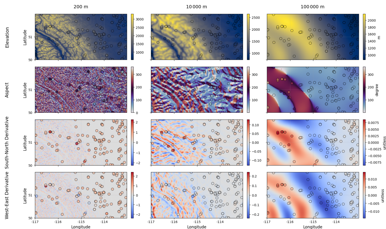
Figure 5. Visual comparison of topographic descriptors used as static predictors in deterministic regression. Calculated based on the MERIT-DEM, and applying a 2D Gaussian filter of varying radii (200, 10 000, and 100 000 m) examples for DEM, Aspect, South-North and West-East Derivatives are shown. Station location and values derived from the gridded products are indicated within the circles.
