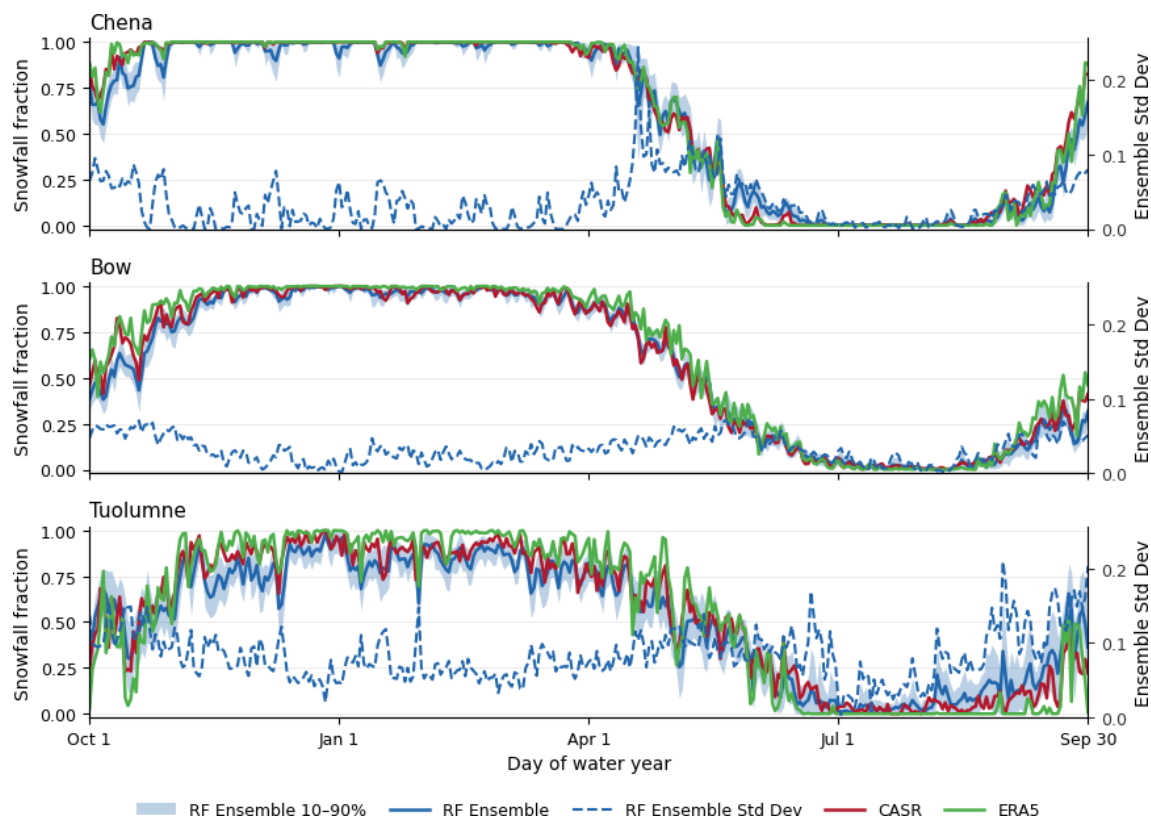
Figure 15. Snowfall fraction (fraction of precipitation that falls as snow) displayed across the water year, including the ensemble spread and standard deviation of ensemble runs.
