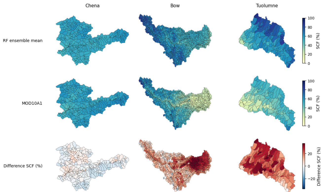
Figure D1. Snow Cover Fraction (SCF) averaged over all water years (2010–2018). This plot shows the RF ensemble mean result, the MODIS measurement, and the difference between them. Snow Cover Fraction (SCF) is overestimated in lower elevation sub-basins in both the Bow and the Tuolumne. This would contribute to an overestimation in catchment mean. Chena results are more consistent spatially and show closer agreement between model and measurements.
