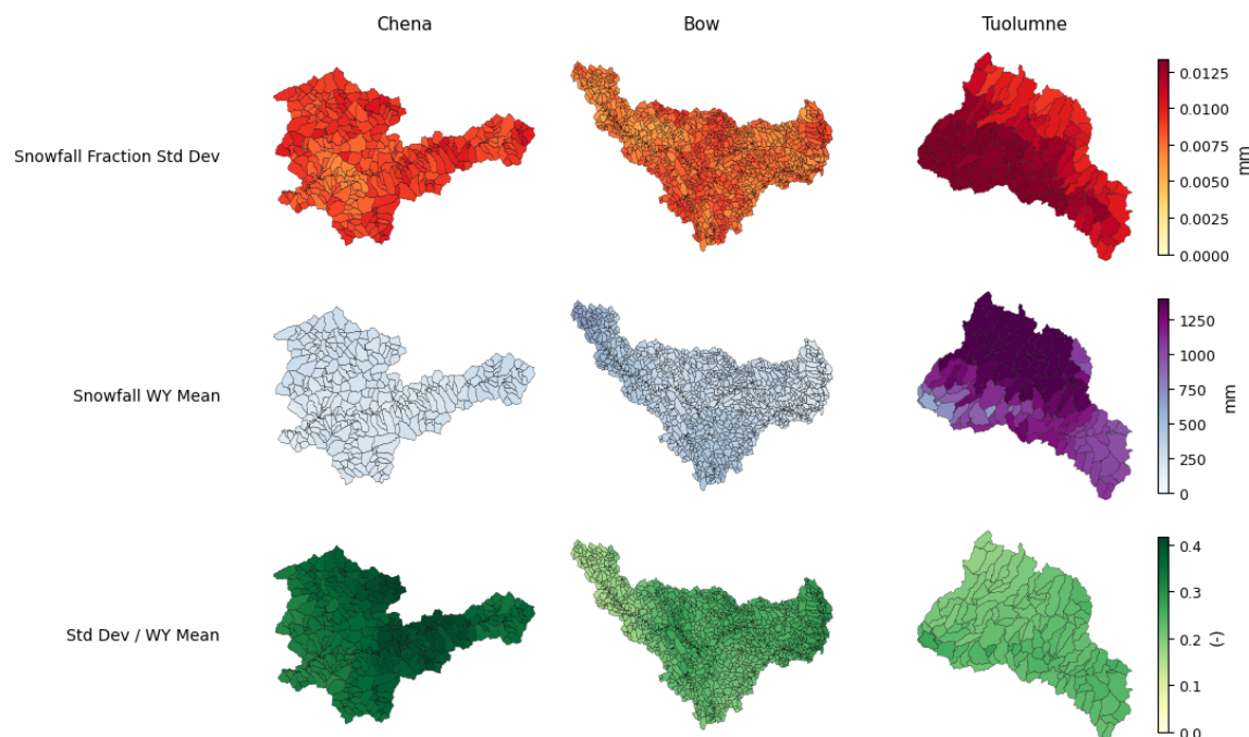
Figure D3. Snowfall fraction is calculated across ensemble members and the standard deviation used to represent precipitation phase uncertainty. The uncertainty in precipitation phase across the simulation period does not indicate a distinct spatial pattern, with the exception of high uncertainty at Tuolumne lower elevations. Normalizing the standard deviation by the total mean water-year snowfall allows comparison across basins.
