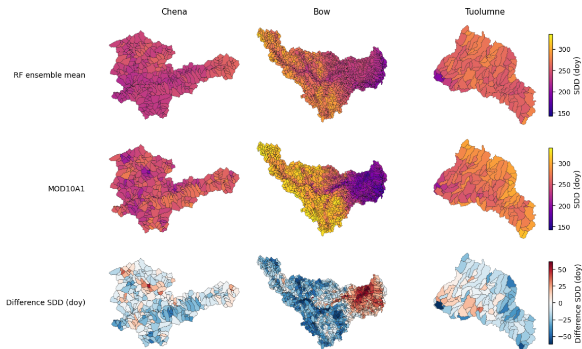
Figure D2. Snow Disappearance Date (SDD) averaged over all water years (2010–2018). This plot shows the RF ensemble mean result, the MODIS measurement and difference between. Comparable to the SCF result, the SDD is overestimated in the lower elevations for Bow and Tuolumne while the upper elevation sub-basin SDD tends to be more underestimated by the model.
