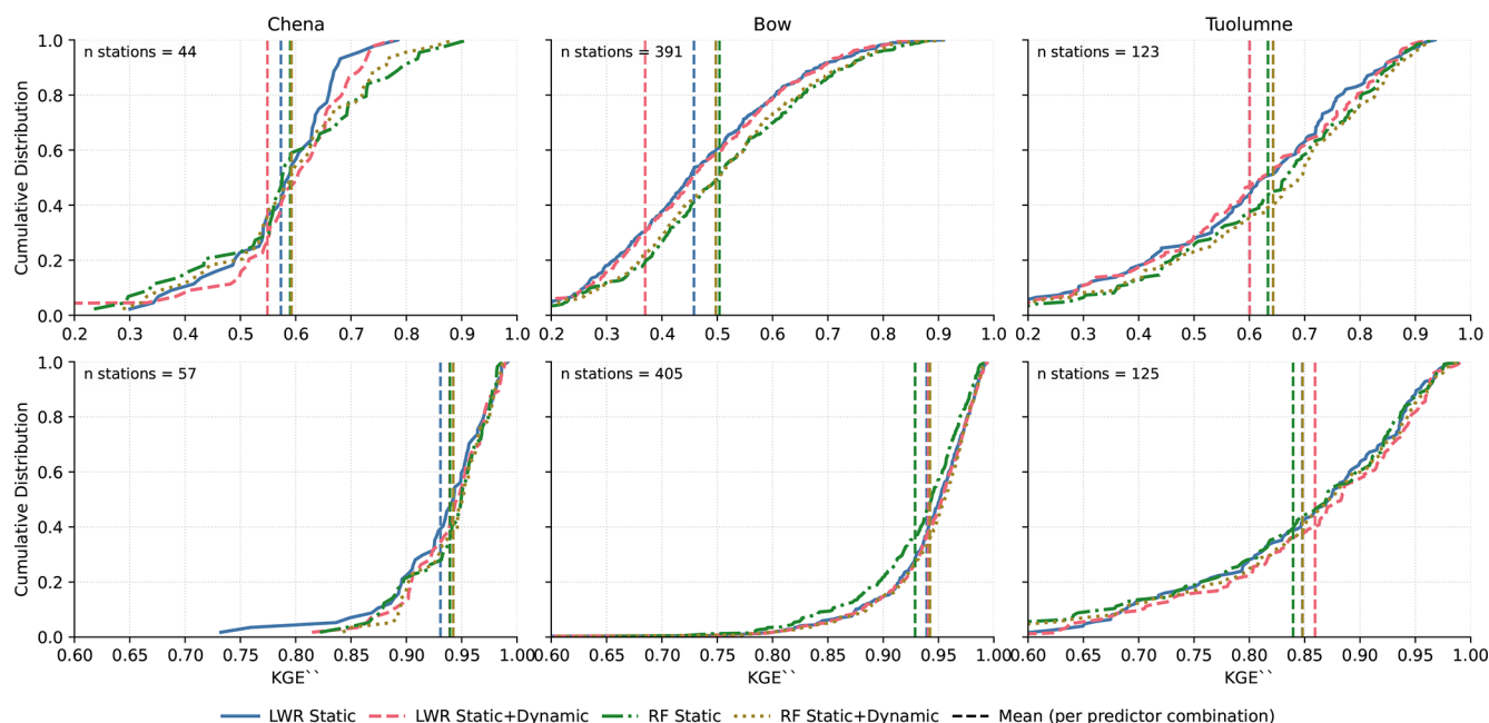
Figure 8. Cross-validation KGE'' values for predictor combinations from forward screens. The KGE'' for all stations are shown as a cumulative distribution function. Results further to the right of the x -axis are better. The number of stations available for each analysis is shown.
