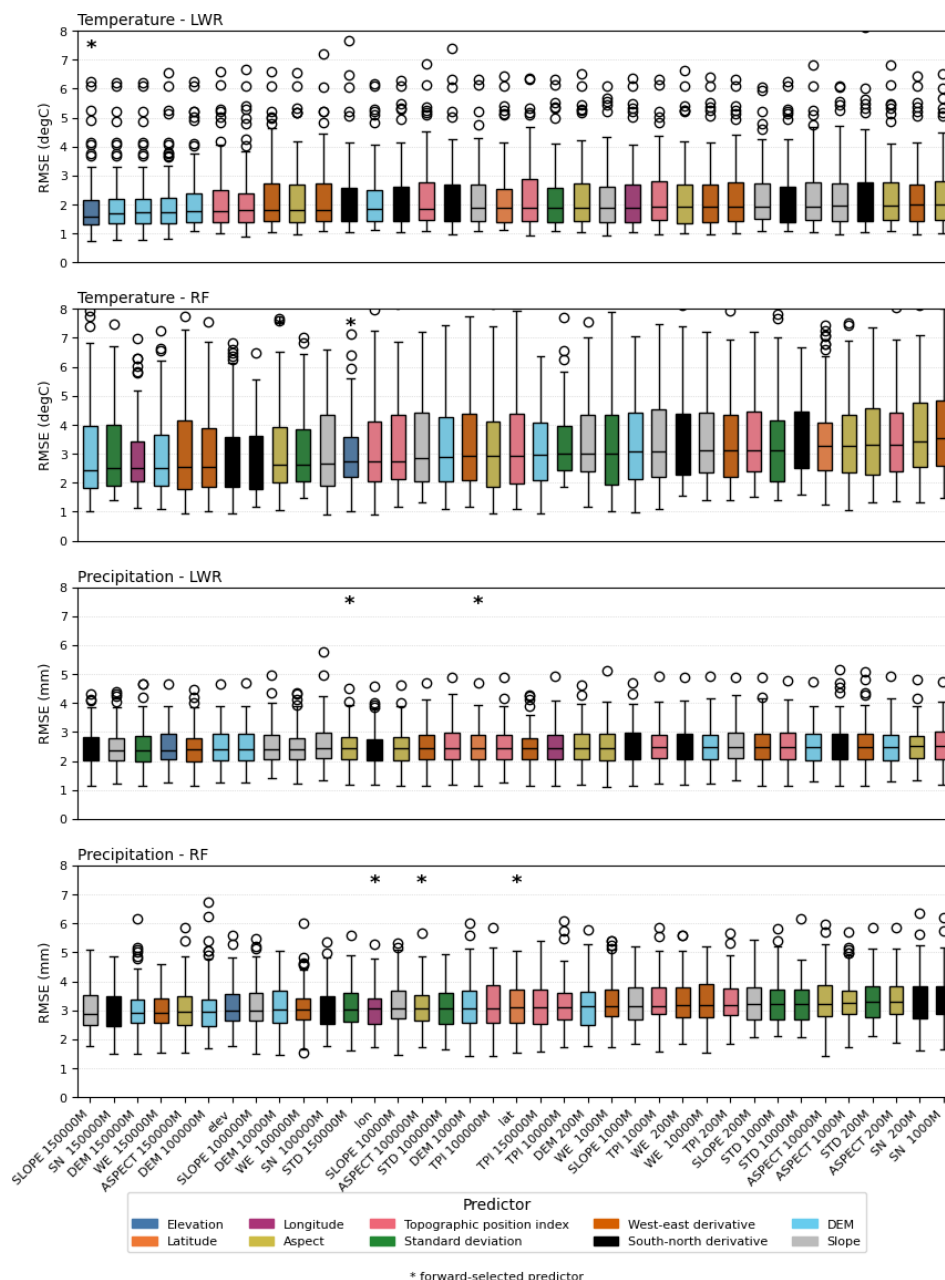
Figure 7. Static predictor screening showing single predictor cross-validation results for the Bow. Topographic descriptors and their smoothed variants (200, 1000, 10000, 100000, 150000 m) are evaluated to assess cross-validation RMSE for temperature and precipitation for both Locally Weighted Regression (LWR) and Random Forest (RF). Asterisk indicates the predictor retained in sequential forward screening.
