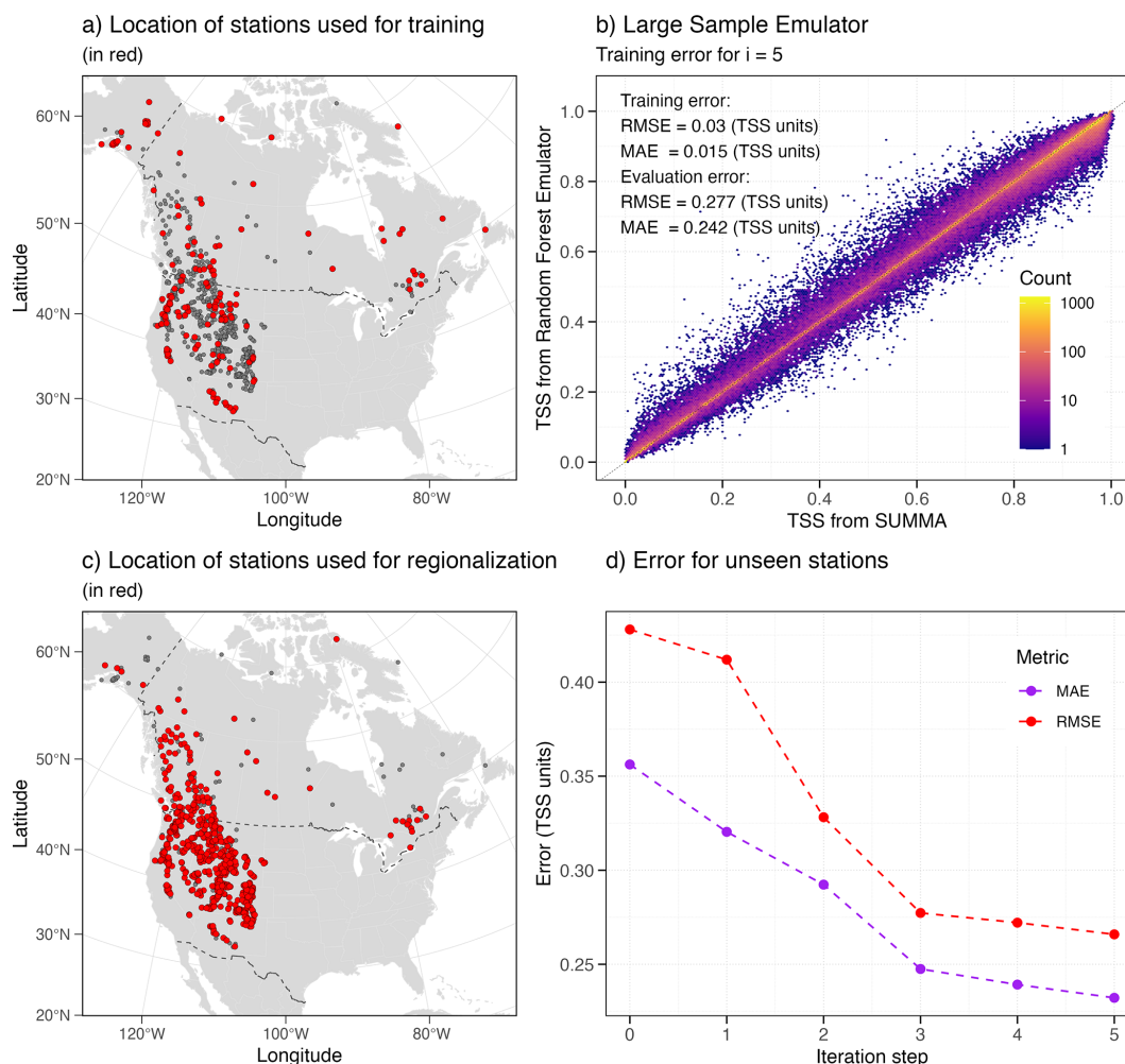
Figure C1. Emulator errors for training and unseen stations. (a) Location of the basins (in red) used to train the emulator ( n = 162 ). (b) Training error for emulator at iteration step i = 5 , and evaluation errors for the new parameter sets obtained through the Genetic Algorithm optimization search. (c) Stations used for parameter regionalization (i.e., unseen stations, n = 608 ). (d) Root Mean Square Error (RMSE) and Mean Absolute Error (MAE) between SUMMA TSS and emulated TSS for the unseen stations and from the emulator trained for each step of the iterative process to refine the emulator.
