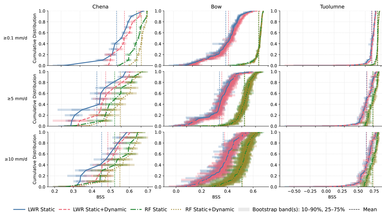
Figure 10. Brier Skill Scores (BSSs) for precipitation with bootstrap resampling. The CDFs of BSSs show the relative performance of each method compared to the climatology mean. BSS = 1 indicates a perfect probabilistic prediction, while all values above 0 are better than the climatology.
