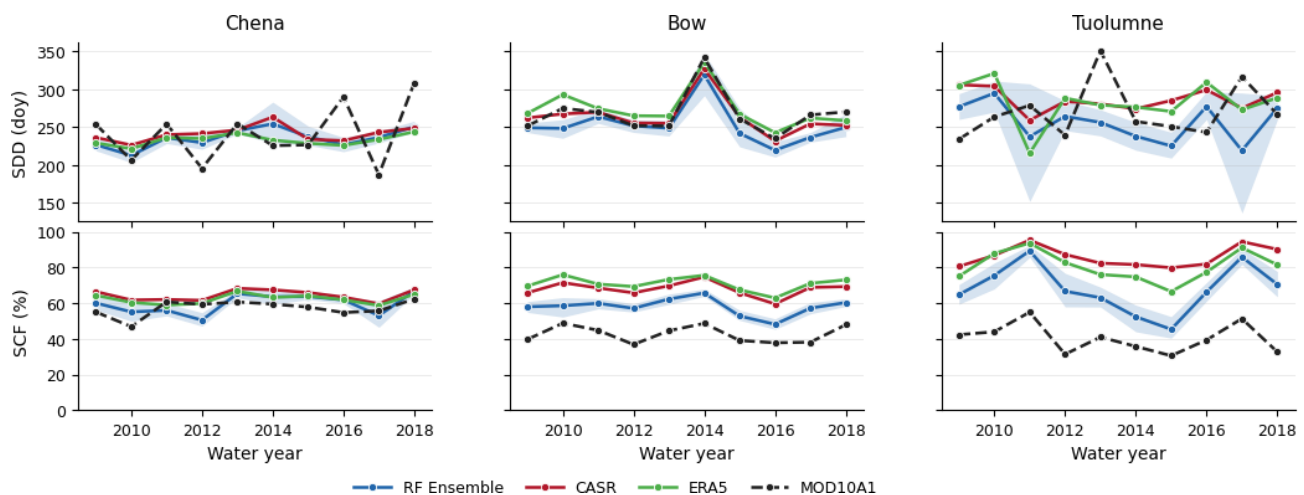
Figure 14. Snow Disappearance Date (SDD) and Snow Cover Fraction (SCF) for snow model results compared to MODIS MOD10A1 derived measurement. Metrics are aggregated spatially over the catchments and calculated for each water year.
