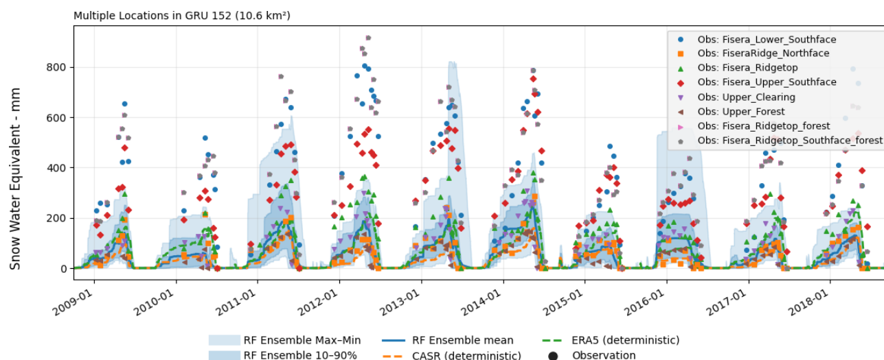
Figure 16. SUMMA SWE simulations of a single GRU with multiple observation sites in the Bow. Measurement location has a large effect on the quantity of snow. This highlights the challenge of evaluation and interpretation of semi-distributed model simulations with in situ data.
