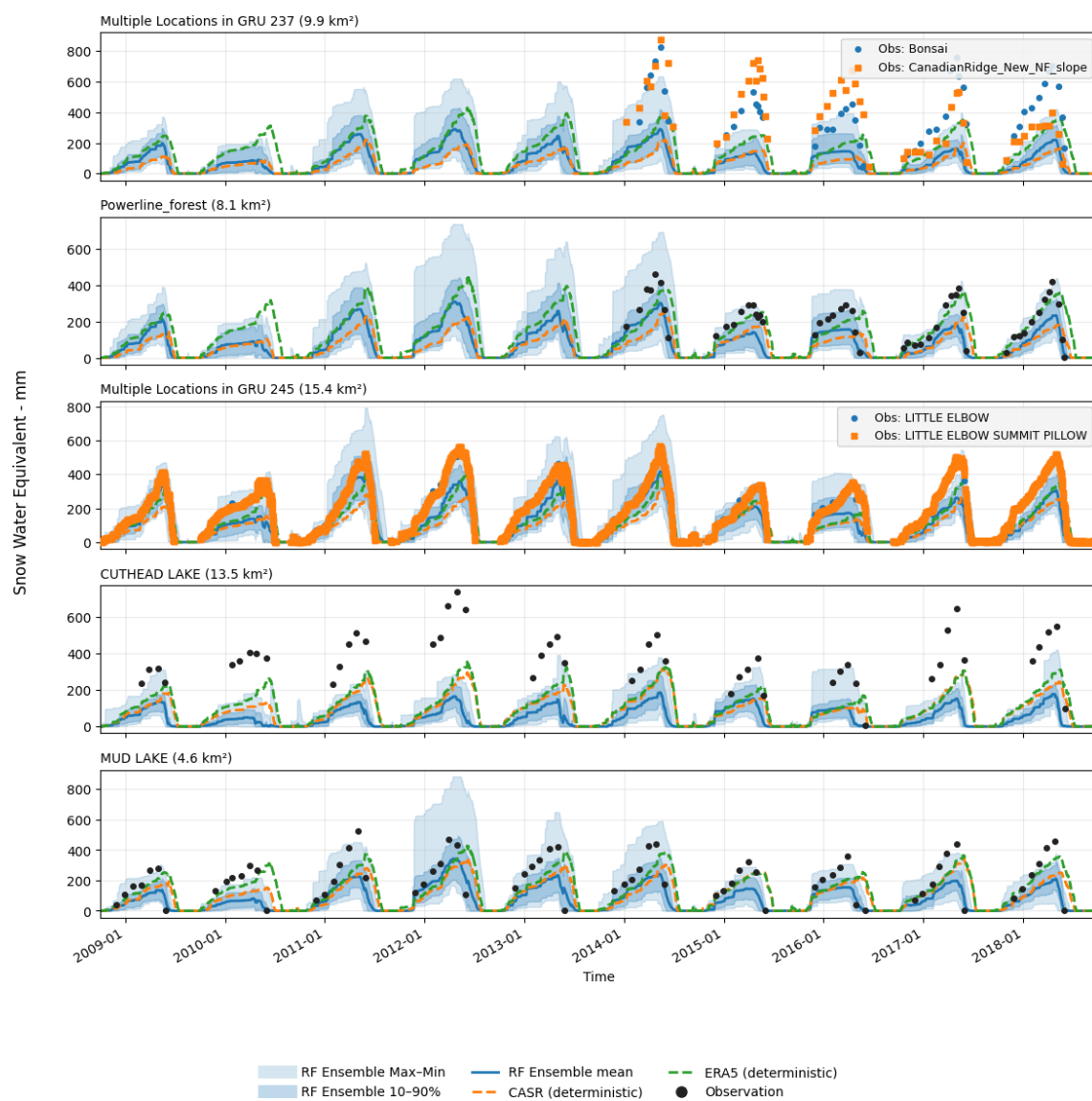
Figure E2. Bow SUMMA Snow Simulation Timeseries compared to NorSWE observations.
