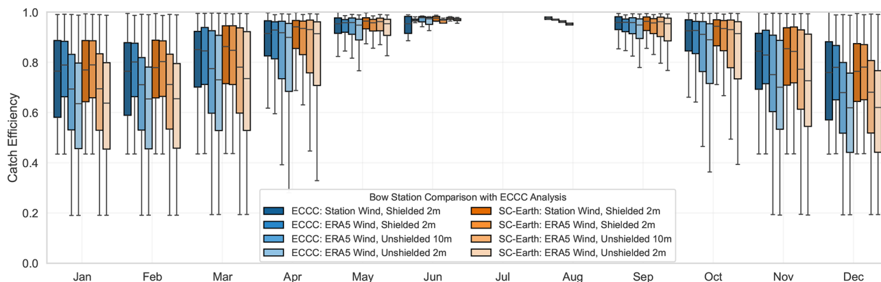
Figure A1. Comparison of methodological choices for undercatch correction using overlapping SC-Earth stations with that of Smith et al. (2022) in the Bow. The shielded 2 m ECCC station dataset represents the reference dataset, while separate iterations assess the effects of supplementing SC-Earth station data with ERA5 winds and applying wind-height corrections.
