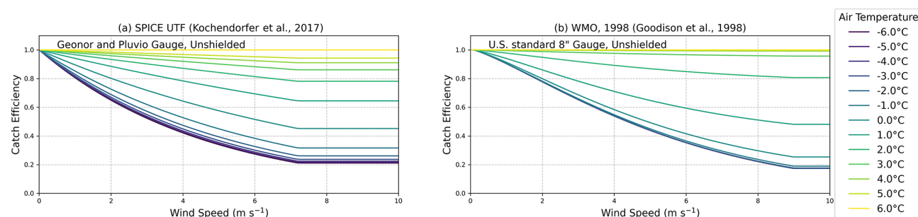
Figure 4. Catch efficiencies for the undercatch correction methods applied in this study based on temperature and wind speed. The updated SPICE UTF Kochendorfer et al. (2017a) to the Bow Basin is shown on the left side (a). On the right side (b) for the Chena and Tuolumne the approach from Goodison et al. (1998) and wind speed threshold behavior from Yang et al. (1998).
