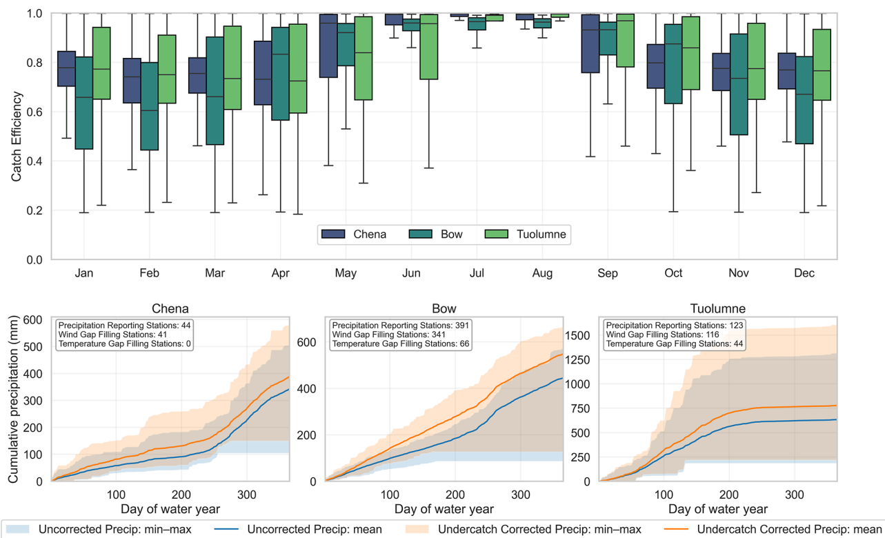
Figure 6. Gauge catch efficiency (CE) and cumulative precipitation across basins. The top panel shows CE correction ranges by month across the Bow, Chena, and Tuolumne basins. The bottom panel shows the effect of undercatch correction on precipitation accumulation over the water year (starting 1 October). Each water year and the mean of all years and stations are shown for each basin. Both the boxplots and area time series summarize calculations at station locations grouped by basin.
