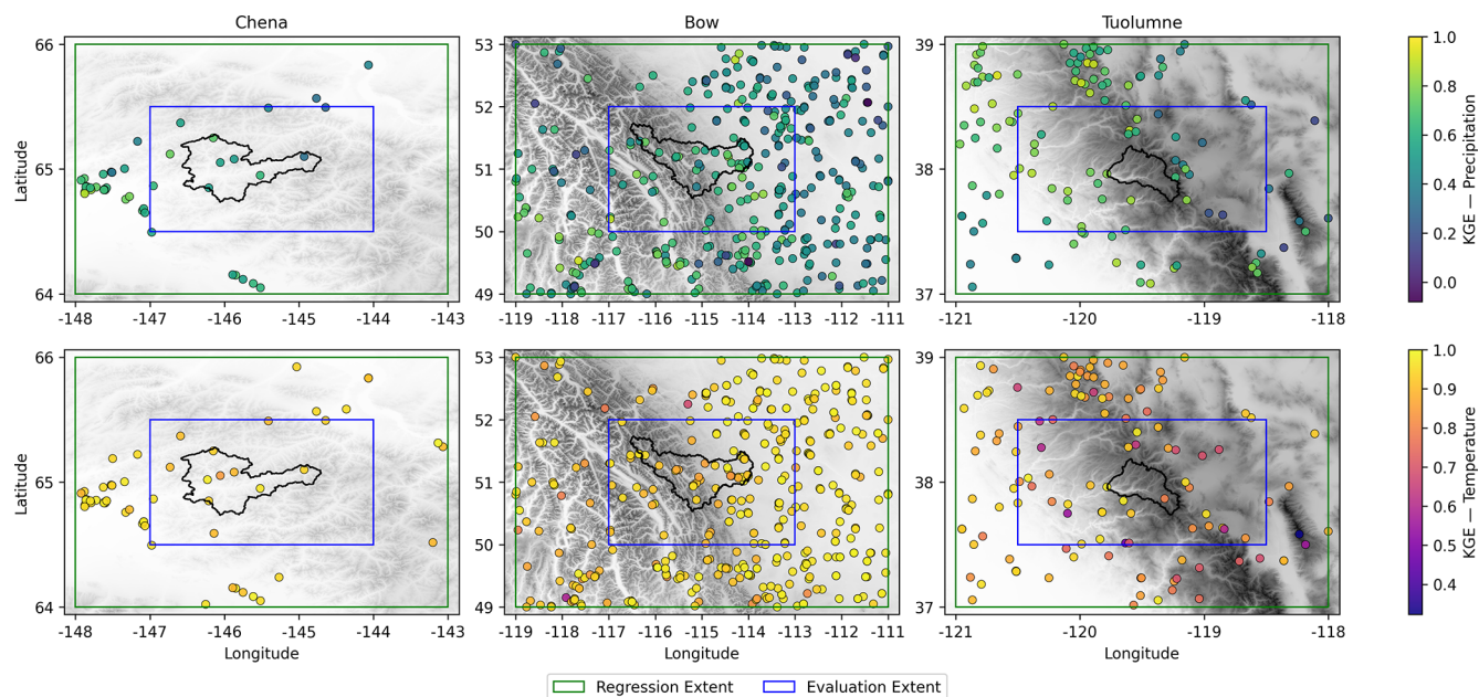
Figure 9. Cross-validation results for Chena, Bow, and Tuolumne River Basins shown as spatial plots for the RF (Random Forest) static and dynamic predictor combinations. Not all stations have both precipitation and temperature measurements. The background map represents elevation.
