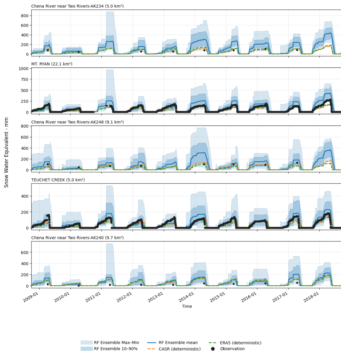
Figure E1. Chena SUMMA Snow Simulation Timeseries compared to NorSWE observations.
