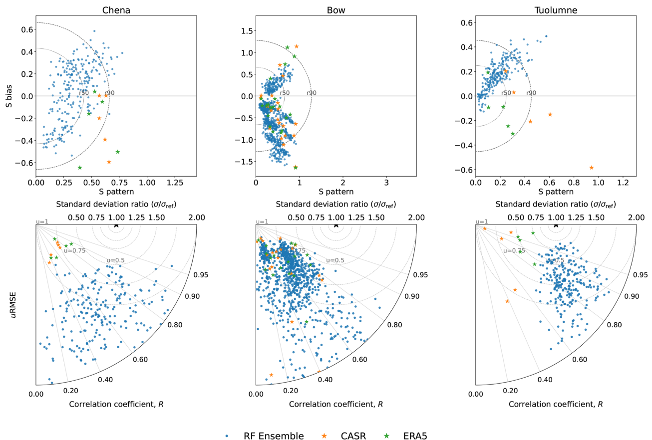
Figure 13. Evaluation of SWE simulations for forcing datasets (Ensemble produced with RF Static–Dynamic predictors ( n = 50 ), CaSR, and ERA5) using the skill-target (top row) and Taylor diagram (bottom row). Each point represents a single GRU–forcing pairing (and ensemble member for the RF ensembles). The skill-target diagrams (top) display normalized bias ( S bias) versus normalized pattern ( S pattern) relative to snow observations; the dashed circles denote 50th and 90th percentiles. Closer to the target origin at zero indicates better performance. The Taylor diagrams (bottom) summarize the same statistics in polar coordinates, with the azimuthal angle representing correlation ( R ), the radial distance showing normalized standard deviation ( S pattern), and contours of equal centered RMSE ( u ) (Taylor, 2001). Together, the two panels quantify relative skill, bias and correlation consistency following the benchmarking protocol described in Mudryk et al. (2025).
