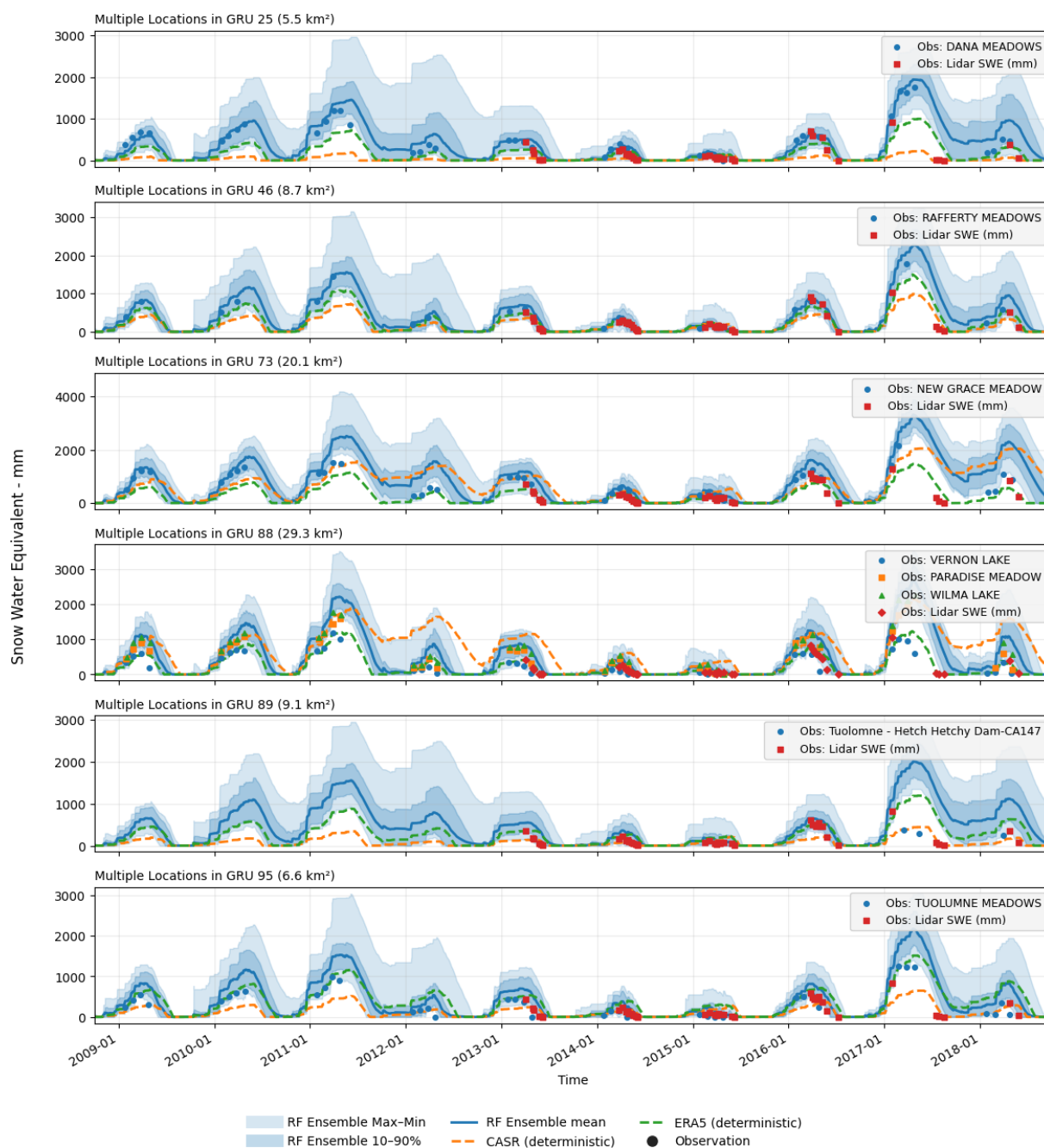
Figure E3. Tuolumne SUMMA Snow Simulation Timeseries compared to NorSWE observations. ASO lidar estimates of SWE are also shown as sub-basin averages from 2014–2018.
