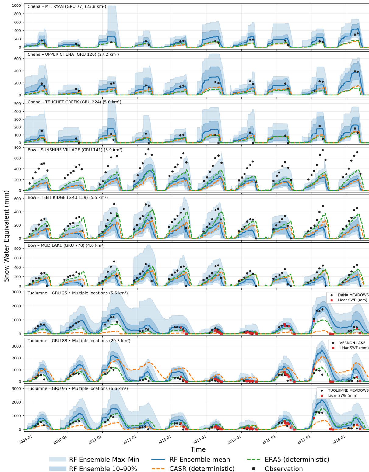
Figure 12. SUMMA sub-basin snow simulations compared to snow surveys. Snow model simulations for the Chena, Bow and Tuolumne are plotted for RF ensembles, CASR, and ERA5 forcing. For each basin the 3 GRUs with the highest amount of snow survey data are shown. For the Tuolumne, lidar SWE estimates averaged over the GRUs are shown.
